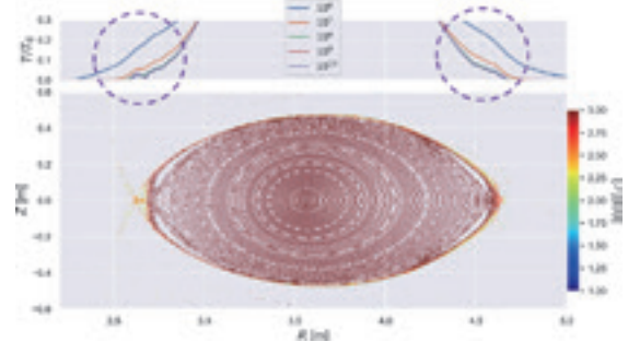
Fig. 1: A comparison of the anisotropic heat diffusion with the different \chi_\parallel/\chi_\perp is shown. The \chi_\parallel/\chi_\perp is scanned from 10^6 to 10^{10} . A top panel shows enlarged T/T_0 profiles on Z = \text{const.} plane, and a bottom panel shows a Poincaré plot at the horizontally elongated cross section for the vacuum standard configuration. Two purple circles indicate the stochastic magnetic field region. Due to the increased \chi_\parallel/\chi_\perp , the T/T_0 profile is changed.
