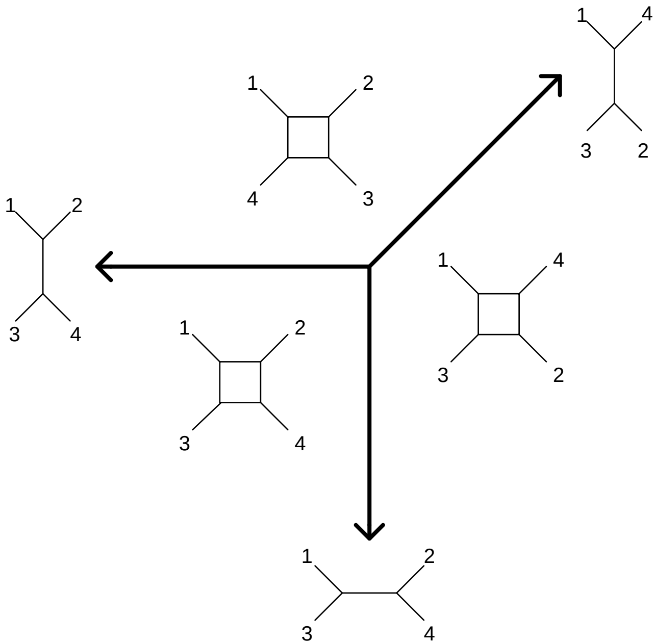
图 5: reduced tropical Grassmannian \mathcal{G}''_{2,4}
