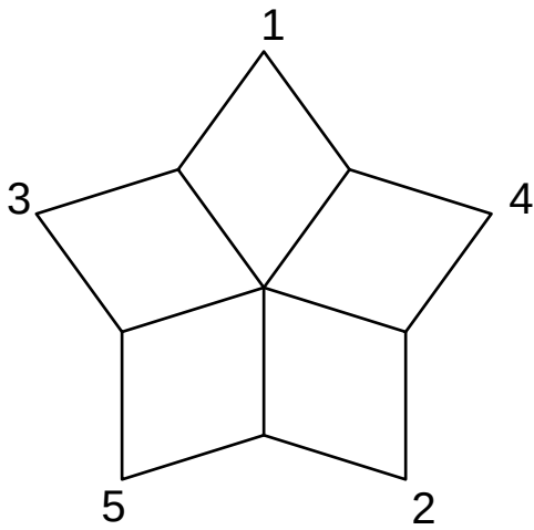
Fig 8: Network in \overline{\mathcal{N}}_5
