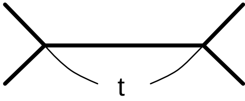
Fig 6: Phylogenetic tree parametrized by \mathcal{G}_{2,4}
