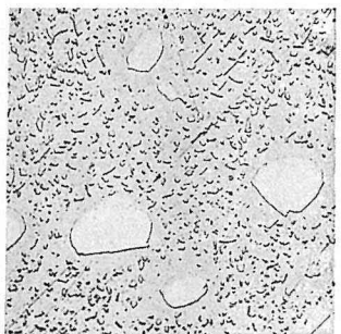
Photo 12. 7.0% Al Quenched from 650°C in boiling water.
