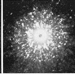
Photo 34. 6.5% Al, 1.0% Sn (Transversal section)
