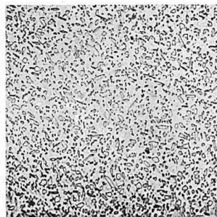
Photo 11. 7.0% Al Quenched from 680°C in boiling water.
