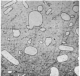
Photo 6. 7.0% Al Quenched from 630°C in ice-water.
