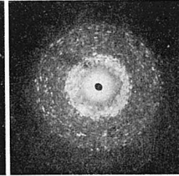
Photo 38. 6.5% Al, 1.0% Sb (Transversal section)
