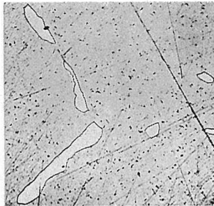
Photo 5. 7.0% Al Quenched from 660°C in ice-water.
