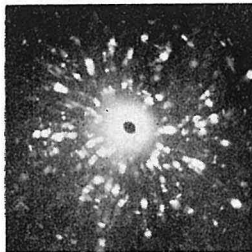
Photo 36. 6.5% Al, 2.0% Sn (Transversal section)
