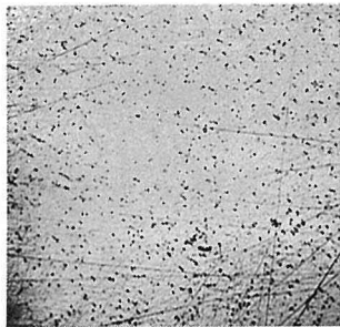
Photo 4. 7.0% Al Quenched from 670°C in ice-water.
