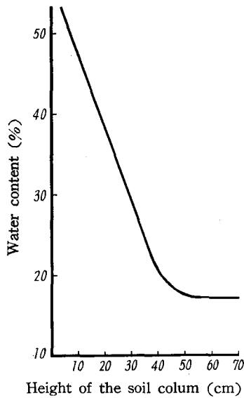
Fig. 2-2 Relation between the height of soil column and the water content (per weight) when full absorbed the water from the base of soil column (full-ed red soil)
