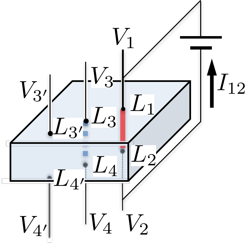
Figure 4.7: Experimental setup for the nonlocal transport due to the TCME. The thick red solid (blue dashed) line represents the (anti-)dislocation line. The leads are attached at the black points, L_i (i = 1, 2, 3, 4, 3', 4') . The line L_1L_2, L_3L_4, and L_{3'}L_{4'} are parallel and have the same length. Here we suppose L_1L_3 < L_1L_{3'} . V_i is the voltage at L_i , and I_{12} is the current. Reproduced from Ref.[20].
