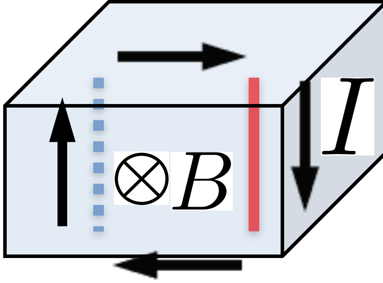
Figure 4.6: The current (shown as arrows and I ) due to the TCME in the presence of a pair of dislocation lines. The thick red solid (blue dashed) line represents the (anti-)dislocation line. We can detect the magnetic field, B , via a scanning SQUID measurement.
