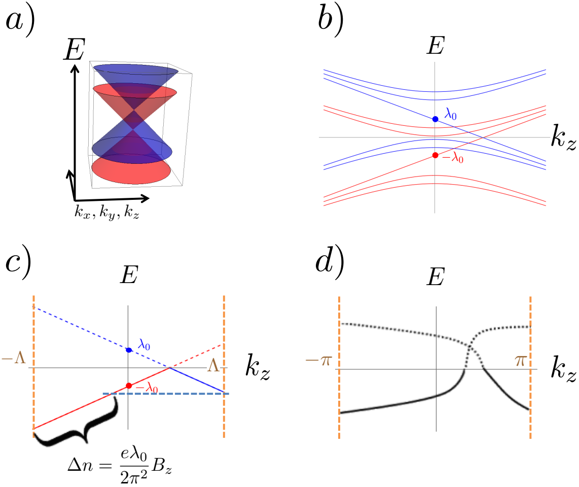
Figure 1.4: a) Band structure of the WSM with broken inversion-symmetry. b) Full spectrum of the WSM in the presence of a uniform magnetic field parallel to the z -axis. c) Chiral modes due to the parity anomaly. d) Band structure of a realistic lattice system. In Figs.c and d, the solid lines and curves represent occupied bands and dashed ones valence bands.
