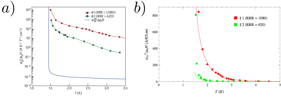
Figure 1.7: a) Transverse Peltier coefficients of URu 2 Si 2 samples with different purities (red dots for a RRR = 1080 sample and green for RRR = 620 one). The solid line is the calculated result based on the Aslamazov-Larkin mechanism. b) Theoretical results of transverse Peltier coefficients due to the chiral fluctuation mechanism [30] (solid lines), which successfully explain the experimental data (circles). These figures are reproduced from Ref.[29].
