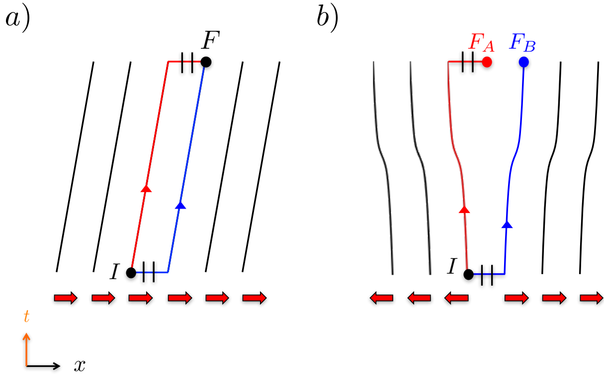
Figure 2.5: Dynamics of one-dimensional fluids with a) homogeneous and b) inhomogeneous velocity profiles. The paths of the particles, A (red) and B (blue), are shown in these figures. The horizontal axis is the spatial axis, and the vertical one is the temporal one. The red arrows represent the velocity field. The solid lines are the world-line of particles. In Fig.b, there is a "space-time edge dislocation", which causes a nonzero torsion, T_{0x}^{\bar{x}} .
