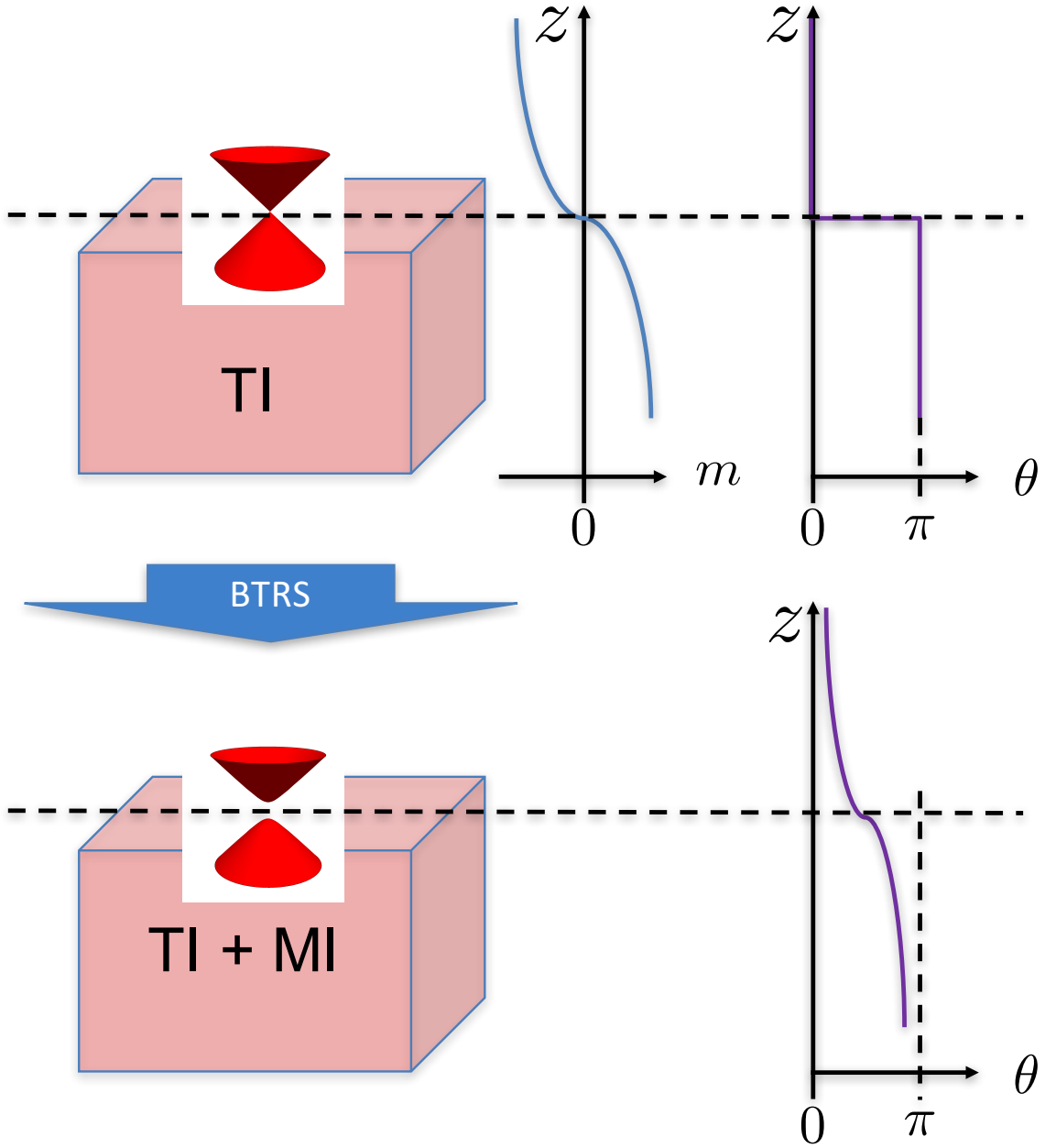
Figure 2.9: Three-dimensional TI, of which surface a two-dimensional massless Dirac fermions (upper figure), and, breaking the time-reversal-symmetry by doping magnetic impurities, they acquire mass and the surface spectrum becomes gapped and therefore the surface corresponds to "one-half of" the CI (lower figure).
