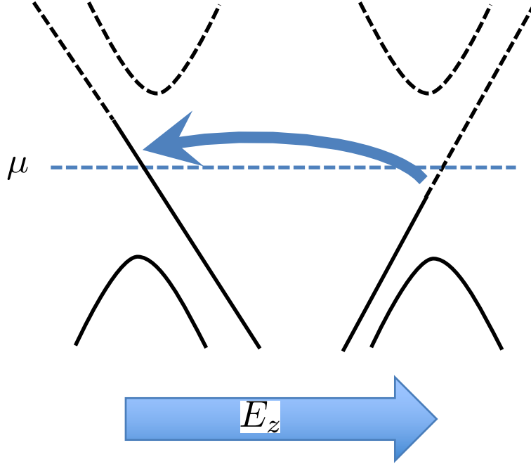
Figure 1.5: Mechanism of the LNMR. \mu is the chemical potential. The solid lines and curves represent occupied bands and dashed ones valence bands.
