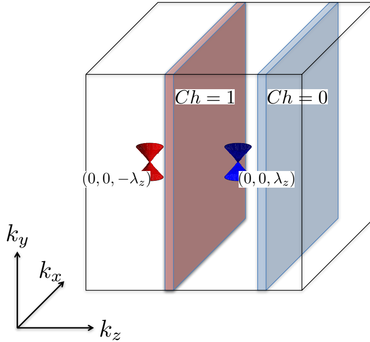
Figure 1.3: BZ of the WSM. The Chern number of a k_x k_y -plane is equal to 1 when this plane is sandwiched by the Weyl points (red plane) and 0 otherwise (blue plane).
