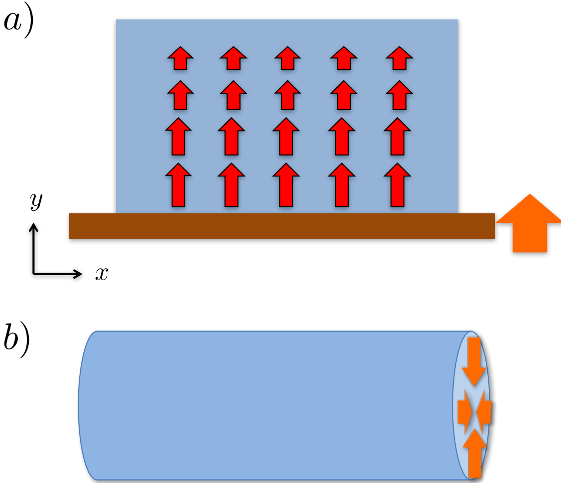
Figure 2.7: Setups for realization of the space-time edge dislocation in a) fluid and b) fluid or lattice systems. Red arrows represent the velocity of the fluid in Fig.a. In Fig.a, the solid domain wall (brown bar) push the fluid and causes density wave, and in fig.b the cylinder is shrunk or enlarged.
