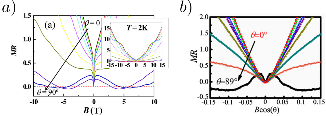
Figure 1.6: Magnetoresistances of (a) \text{Bi}_{1-x}\text{Sb}_x and (b) TaAs. In both case, \theta = 90^\circ corresponds to \mathbf{B} \parallel \mathbf{E} . Reproduced from Refs.[22, 25].
