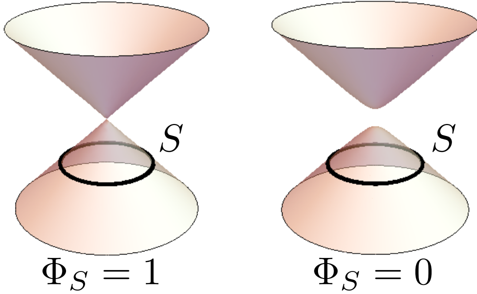
Figure 1.2: Weyl node protected by the topological number. (left) Weyl node, which has the Chern number 1 and (right) gapped state, which has the Chern number 0.
