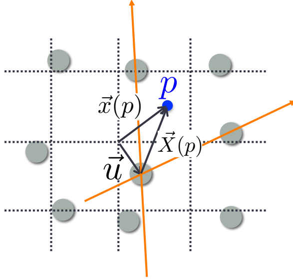
Figure 2.2: Deformed lattice and lattice frame (orange chart). \vec{x}(p) is the coordinate of the point p in the laboratory frame and \vec{X}(p) is that in the lattice frame, and \vec{u} is the displacement vector.
