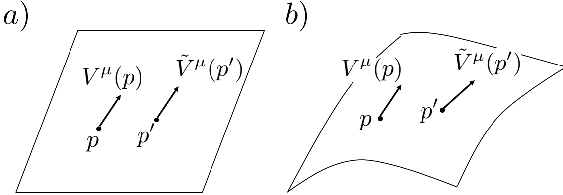
Figure 2.1: Parallel transports of vectors in a) flat and b) curved spacetime.
