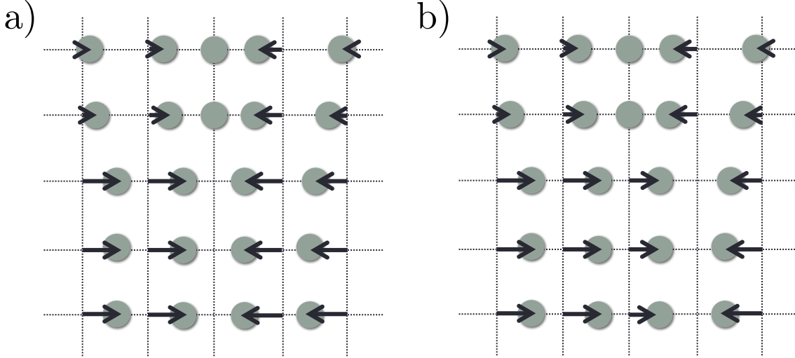
Figure 2.3: Displacement vectors of a lattice with an edge dislocation. a) and b) represent the same lattice but the displacement vectors (arrows) can be defined in different ways. Then the displacement vector field is multivalued.
