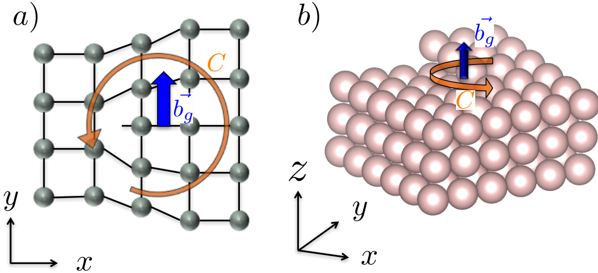
Figure 2.4: Displacement vectors of lattices with a) edge and b) screw dislocations. The orange arrows represent the path of the counter integrals C (see Eq.(2.2.8)), and the blue arrows represent the directions of the Burgers vectors \vec{b}_g .
