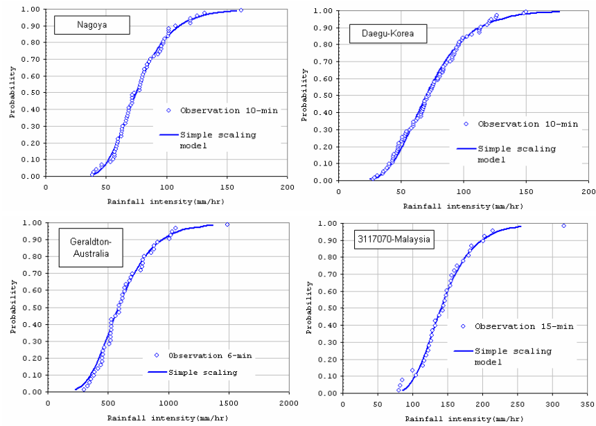
Figure 4 Scaling estimates compared to observation. Circle dot are observation sub-hourly rainfall, the lines are scaling method.
