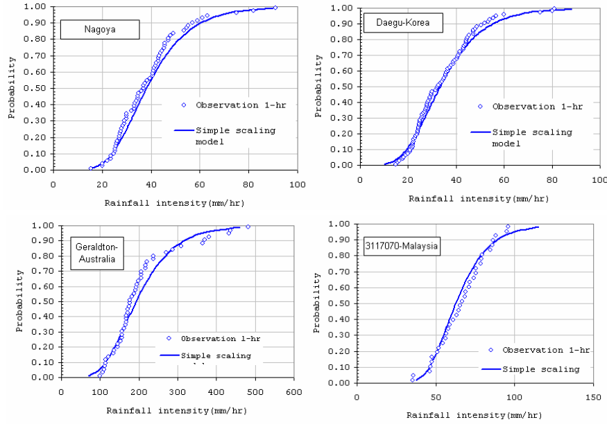
Figure 3 Scaling estimates compared to observation. Circle dot are observation hourly rainfall, the lines are scaling method.
