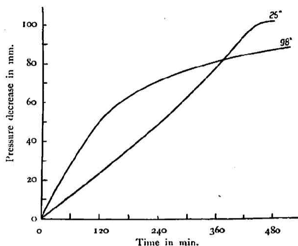
Fig. 9—Experiments with mixtures of C_2H_4 and C_3H_6 : 25°C.-curve, 51.9 mm. C_2H_4 + 49.3 mm. C_3H_6 + 50.3 mm. H_2 ; 98°C.-curve, 53.1 mm. C_2H_4 + 50.7 mm. C_3H_6 + 49.5 mm. H_2 . Time scale for 98°C.-curve is enlarged 4 times.
