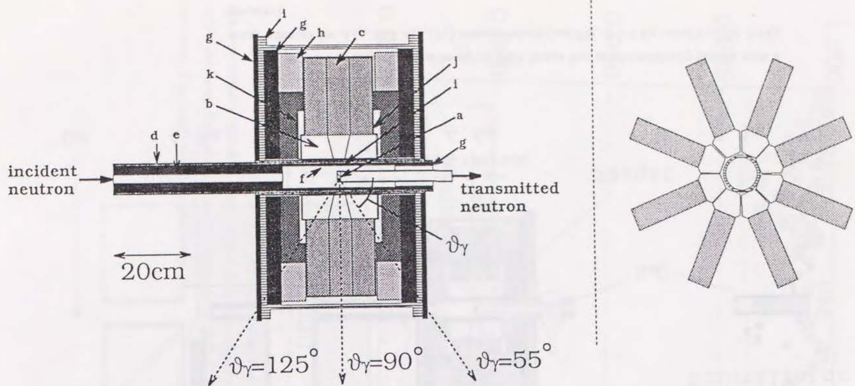
Fig. 4-1-2 Arrangement of BaF_2 \gamma -ray counter for the measurement of the A_{L,\gamma} and the a_{L,\gamma}(\theta_\gamma) . (a)Target, (b) BaF_2 crystals, (c)UV sensitive photomultipliers, (d)50G solenoid, (e) B_4C (neutron absorber), (f)sintered B_4C (neutron absorber), (g) B_4C (neutron absorber), (h)boric acid resin (neutron absorber), (i)iron (magnetic shield), (j) \mu metal (magnetic shield), (k)lead ( \gamma -ray absorber). A cross section of counter configuration seen from down stream on the beam line is shown in the right hand side. The BaF_2 crystals are arranged to detect \gamma -rays at \theta_\gamma = 55^\circ, 90^\circ and 125^\circ . The BaF_2 crystals cover 85% of 4\pi steradians in total.
