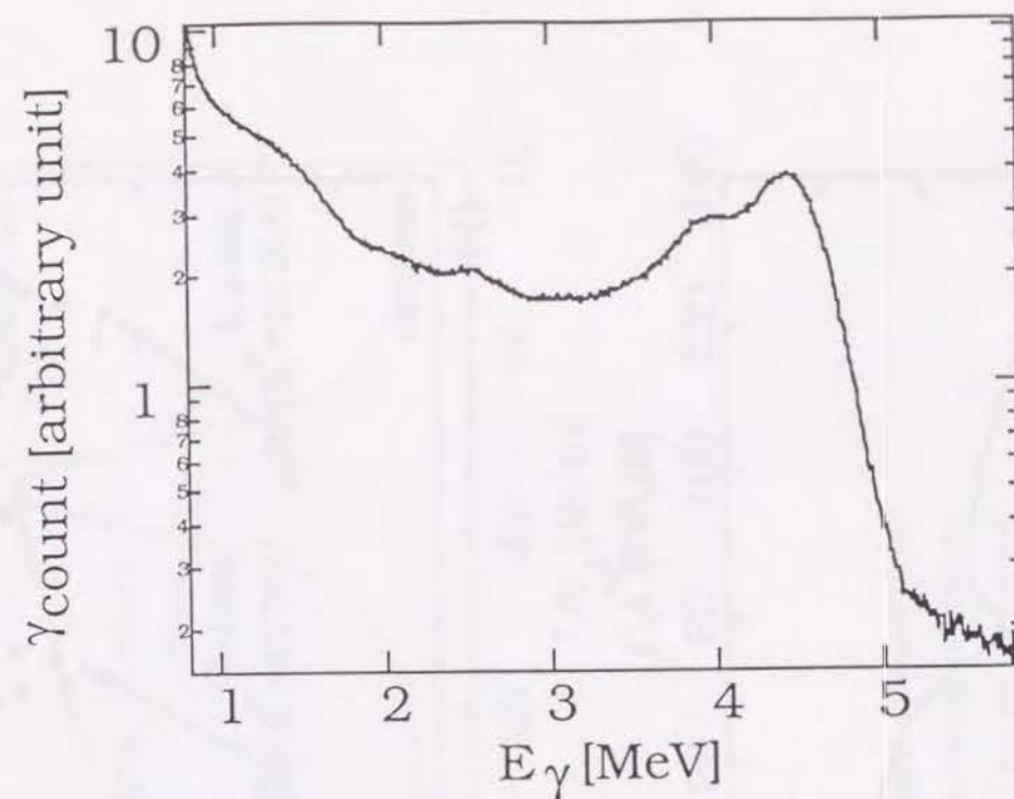
Fig. 4-3-2 A typical pulse height spectrum for \gamma -rays from ^{12}\text{C}^*(4.43\text{MeV}) of Am/Be radioactive source obtained with the BGO counter. The horizontal axis is scaled by fully absorbed \gamma -ray energy. The energy resolution was 13% in FWHM for 4.43MeV \gamma -rays.
