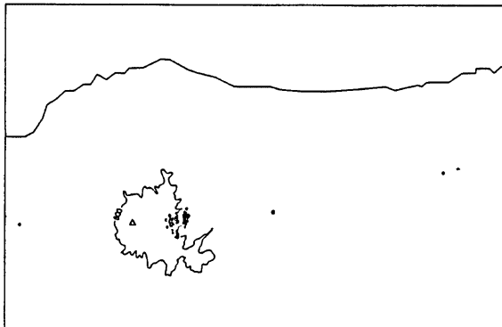
Fig. 3 Epicenters routinely determined by the Tottori Microearthquake Observatory. Upper: before the present swarm. Solid circles indicate M \geq 3 events very near the Daisen. Lower: Present swarm.
