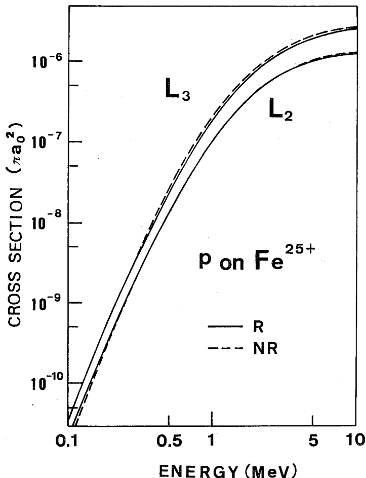
Fig. 2. Cross sections for K-L 2 and K-L 3 excitation of Fe 25+ ion by proton impact. See caption of Fig. 1.
