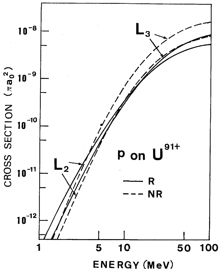
Fig. 4. Cross sections for K-L 2 and K-L 3 excitation of U 91+ ion by proton impact. See caption of Fig. 1.
