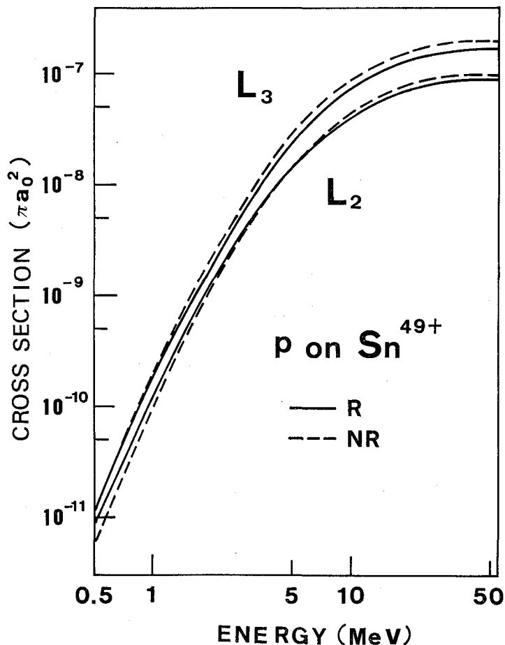
Fig. 3. Cross sections for K-L 2 and K-L 3 excitation of Sn 49+ ion by proton impact. See caption of Fig. 1.
