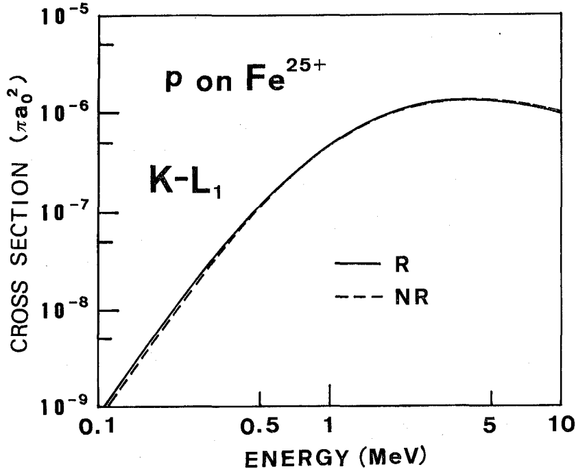
Fig. 1. Cross sections for K-L 1 excitation of Fe 25+ ion by proton impact. The solid curve represents the relativistic cross sections and the dashed curve indicates the nonrelativistic ones.
