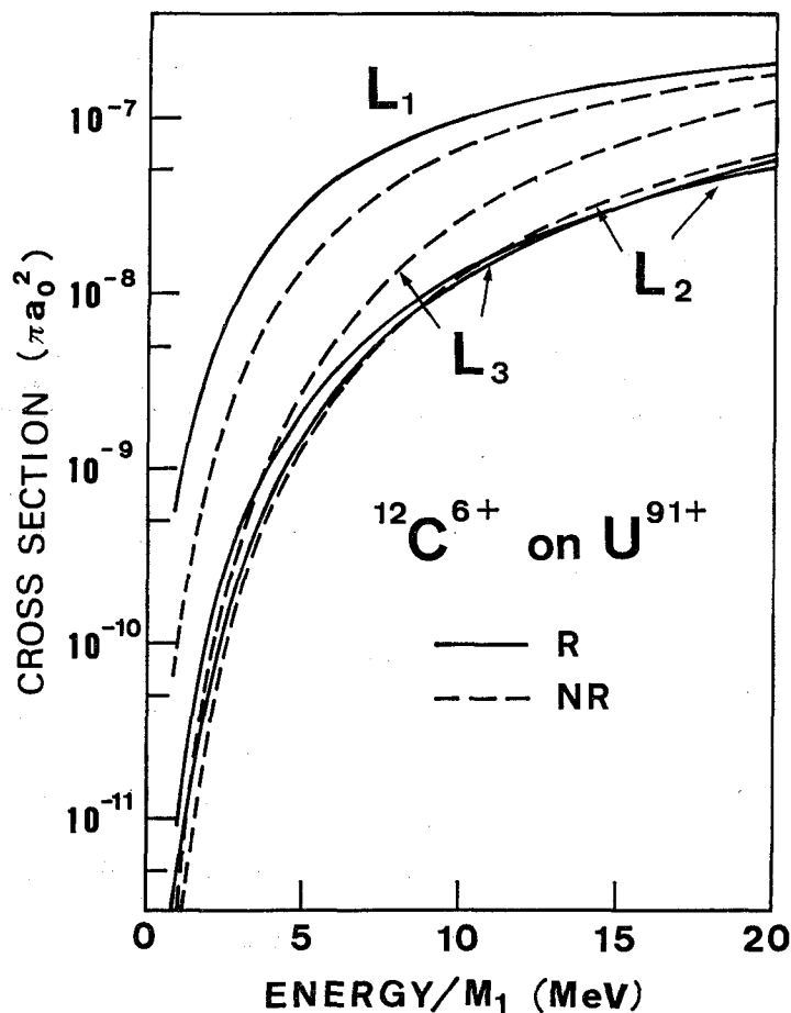
Fig. 5. Cross sections for K-L 1 , K-L 2 , and K-L 3 excitation of U 91+ ion by 12 C 6+ -ion impact. See caption of Fig. 1.
