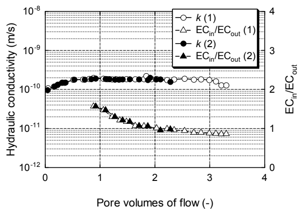
Appendix 24 Changes in k value and EC_{in}/EC_{out} (P-5).
