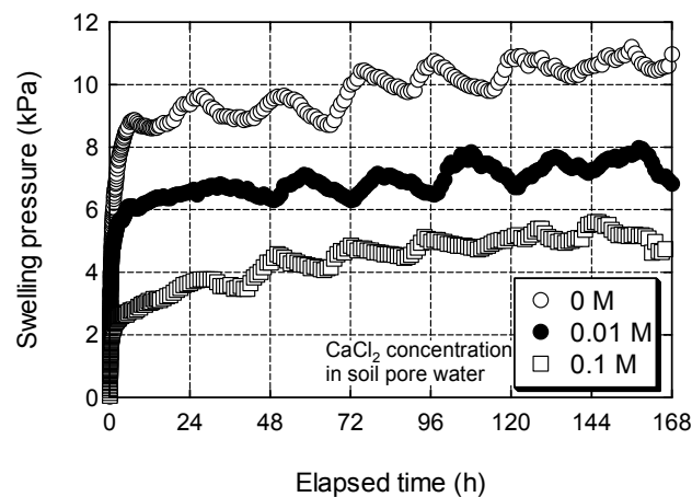
Figure 2.46 Changes in swelling pressure of SBMs with time.
