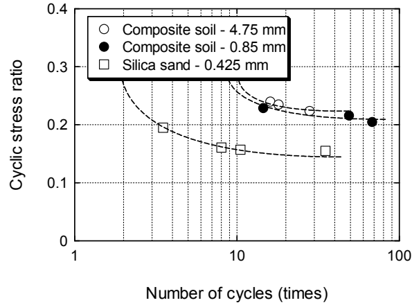
Figure 4.16 Cyclic strength curve at DA = 5\% .
