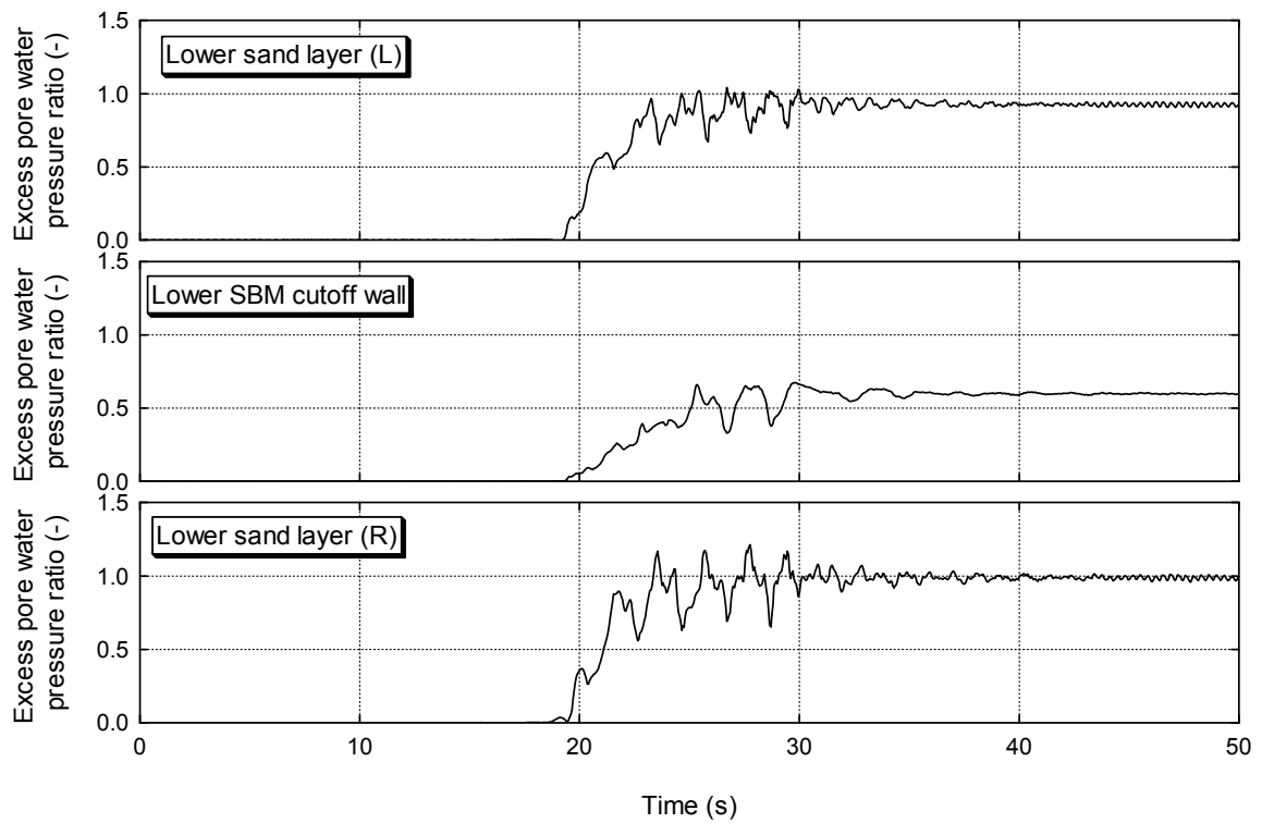
Figure 4.28 Time history of excess pore water pressure ratio (Case-3, at 7.5 m-depth).
