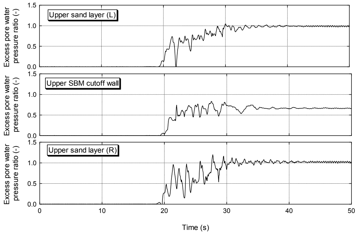
Figure 4.27 Time history of excess pore water pressure ratio (Case-3, at 3.5 m-depth).
