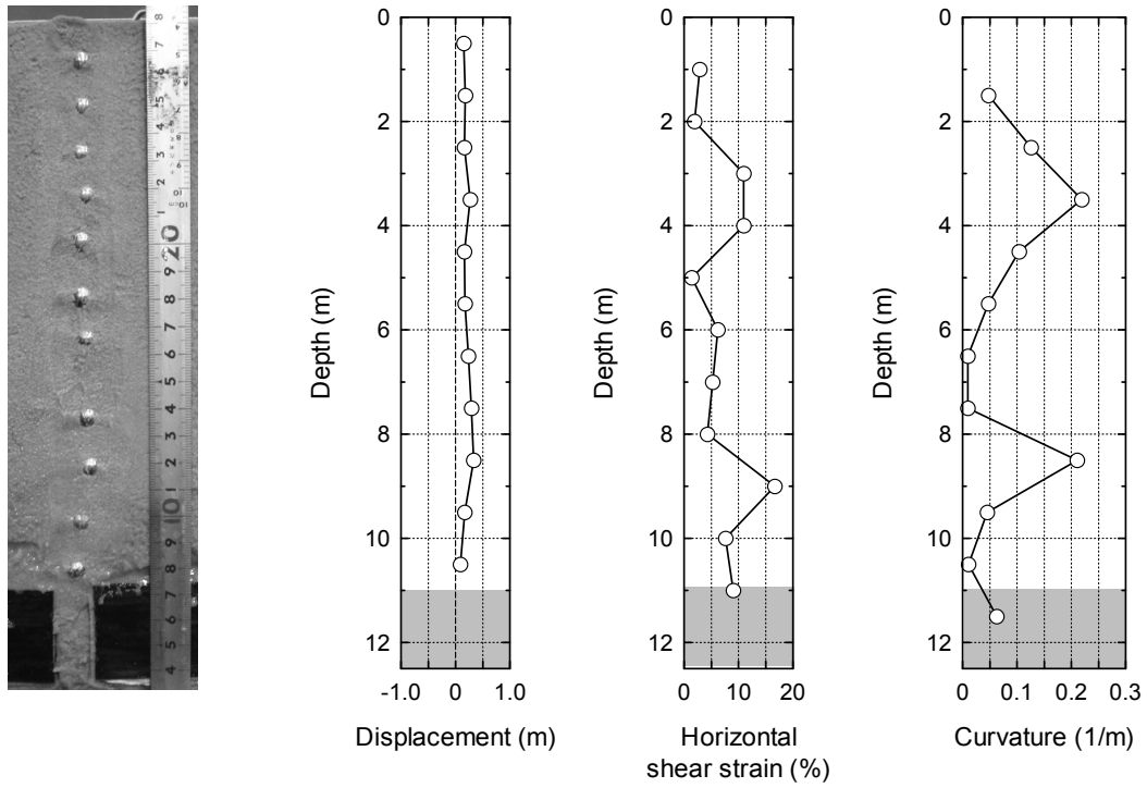
Figure 4.44 Horizontal deformation of SBM cutoff wall in Case-9.
