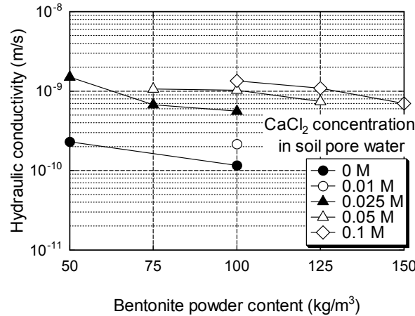
Figure 2.32 Relationship between k values and C_{BP} for each CaCl 2 concentration in soil pore water (P-2, N-1~N-11).
