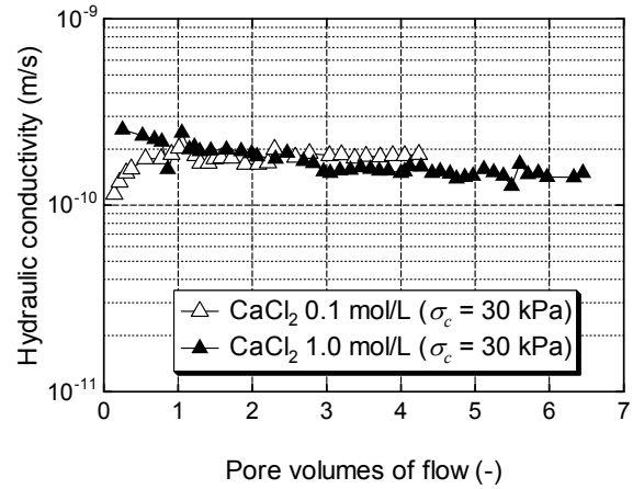
Figure 2.25 Change in the k values with time.
