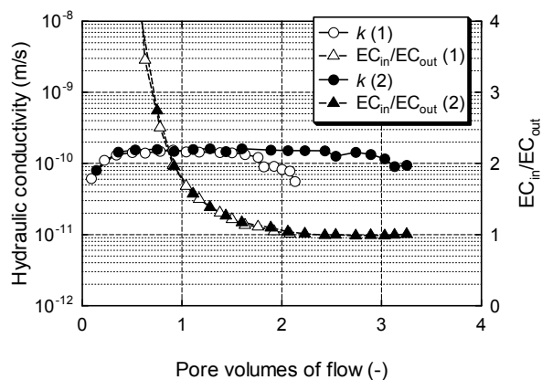
Appendix 26 Changes in k value and EC_{in}/EC_{out} (P-7).
