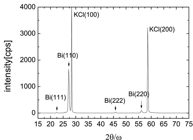
FIG. 2. Typical XRD from the Bi/KCl sample.
