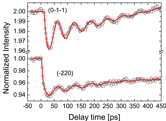
FIG. 4. (Color online) Kinetics of the electron diffraction from (-220) and (0-1-1) for an excitation fluence of \sim 0.9 \text{ mJ/cm}^2 . Open circles represent the experimental data and solid lines are the fitting function.
