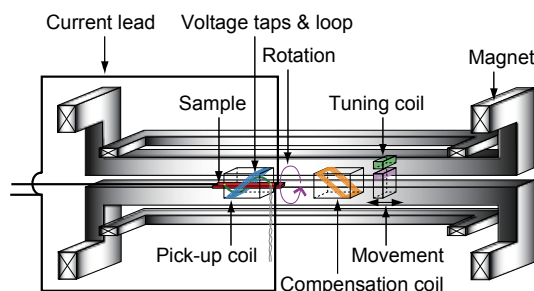
Fig. 6 Experimental set-up for measuring AC loss.
