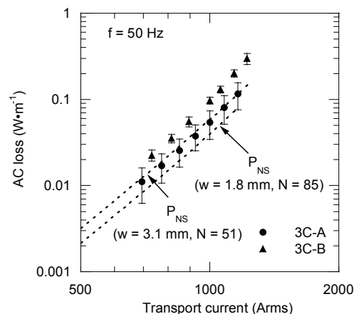
Fig. 25 Measured AC losses of the 1 kA-class multi-layer conductor (3C-A and 3C-B). P_{NS} is the analytical value of Norris's strip model 16) .
