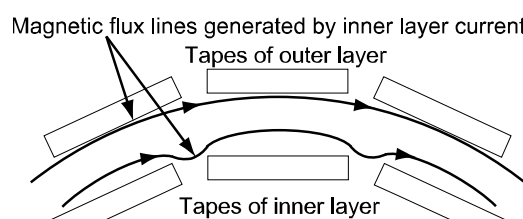
Fig. 23 Schematic of magnetic flux lines in the two-layer cable generated by the inner-layer current.
