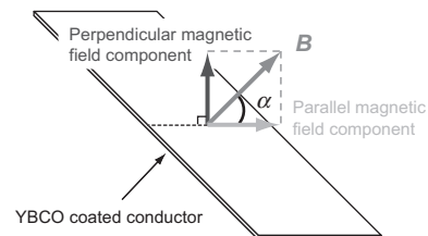
Fig. 11 Thin-strip approximation of the coated conductors for the electromagnetic field analysis.
