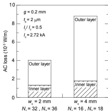
Fig. 24 Calculated AC losses in two-layer cables comprising 2 mm-wide and 4 mm-wide coated conductors, where gap between coated conductors is 0.2 mm.
