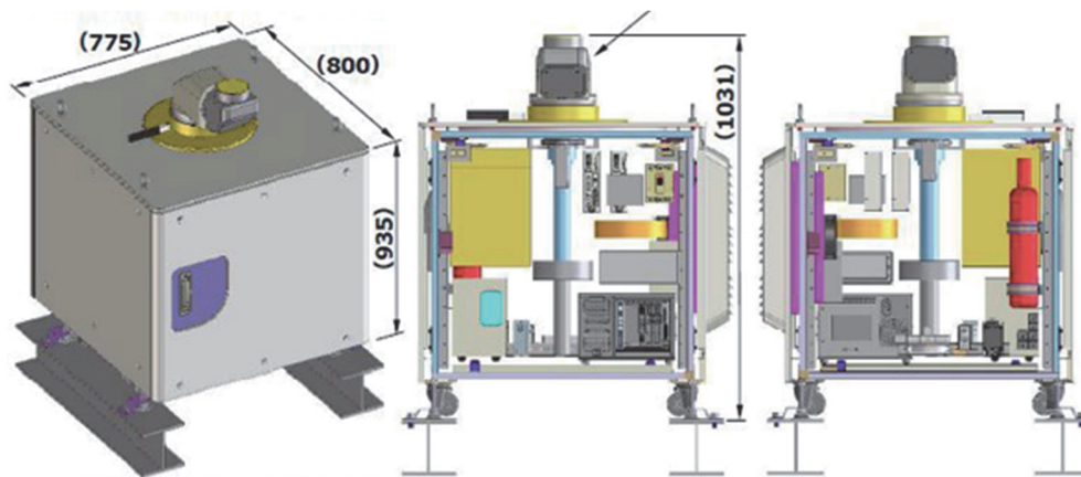
Fig. 1. Coherent Doppler Lidar under development in our laboratory
