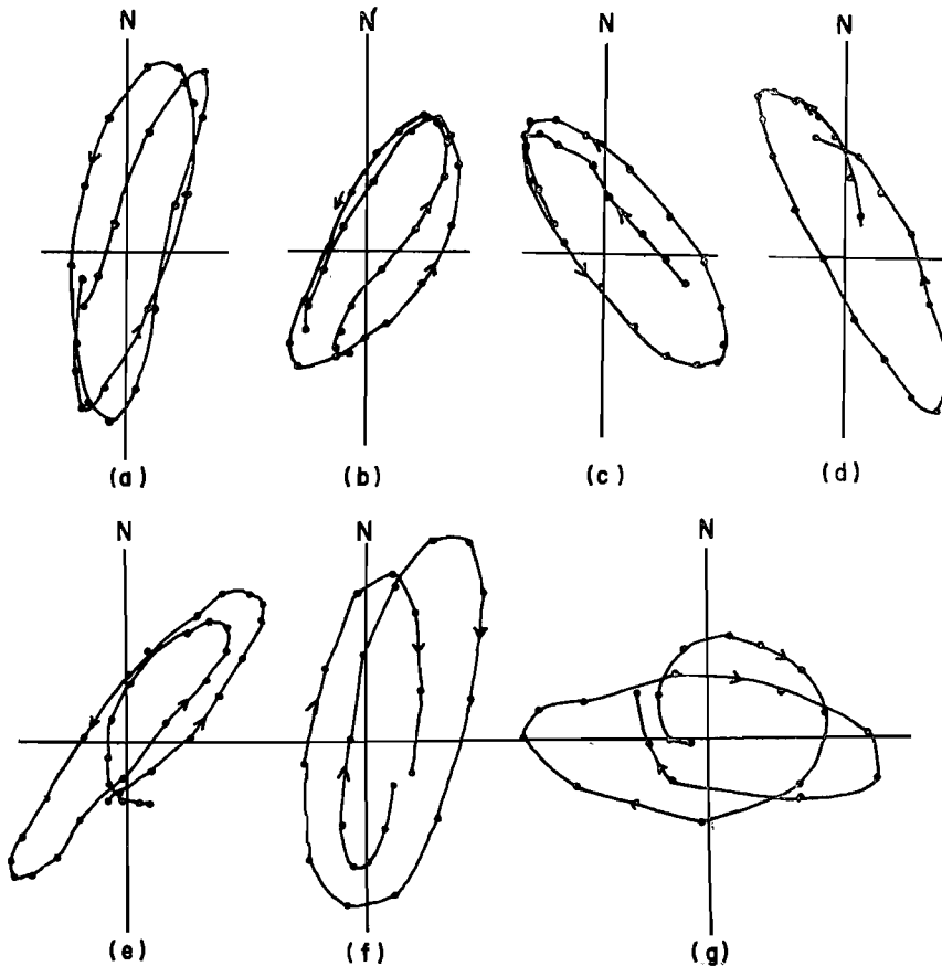
Fig. 8. Typical orbits on horizontal plane of the volcanic micro-tremors of the 1st kind. (a): Vol. Lab., (b): Hakamano, (c): Zigoku-dani, (d): Higashikurokawa, (e): Kusasenri, (f): Sensui-kyo, (g): Hondô.
