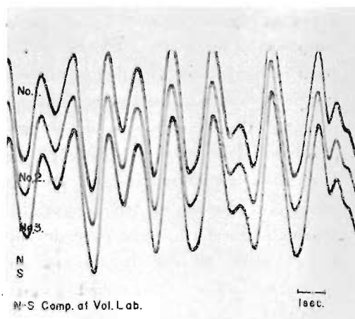
Fig. 2. A portion of the seismogram of comparison of the three horizontal seismographs (SH-2).
