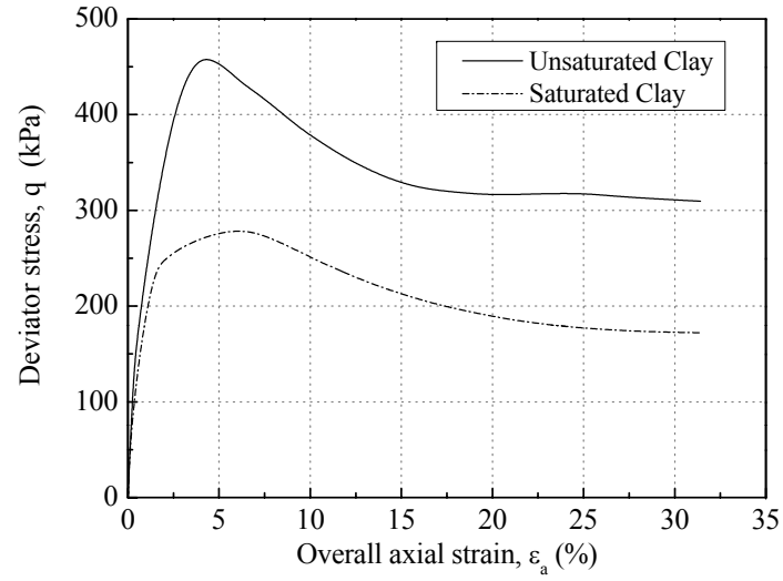
Figure 4.13 Stress-strain relations for unsaturated and saturated clay
