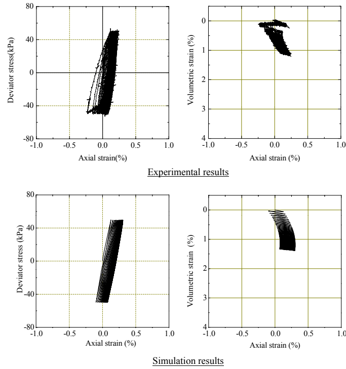
Figure 2.6 Experimental and simulated results for the unsaturated sandy soil under cyclic suction-controlled triaxial conditions (strain rate = 0.01%/min, P^C = 50\text{kPa} )
