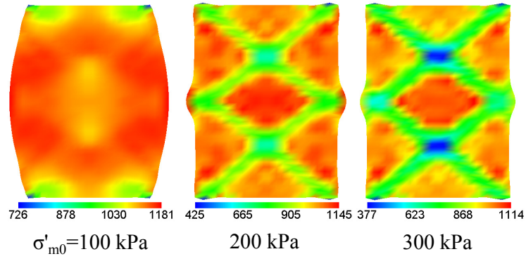
Figure 4.32 Distributions of suction with different initial confining pressures; Unit(kPa); Initial suction P_i^C = 1260 \text{ kPa} , \varepsilon_a = 20\%
