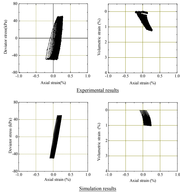
Figure 2.7 Experimental and simulated results for the unsaturated sandy soil under cyclic suction-controlled triaxial conditions (strain rate = 0.1%/min, P^C = 50\text{kPa} )
