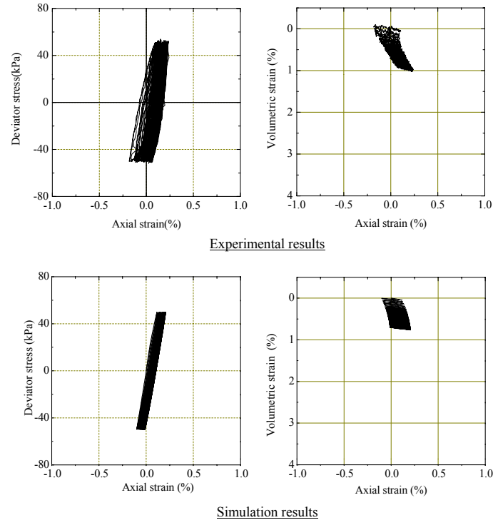
Figure 2.8 Experimental and simulated results for the unsaturated sandy soil under cyclic suction-controlled triaxial conditions (strain rate = 0.75\%/min , P^C = 50\text{kPa} )
