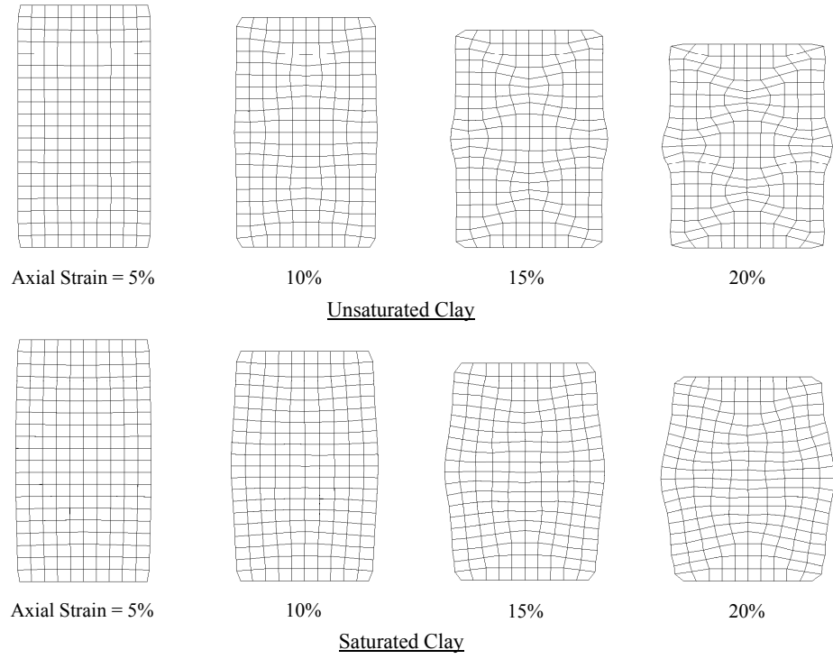
Figure 4.6 Deformed meshes of the specimen at various strain levels for unsaturated and saturated clays
