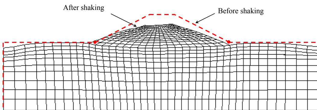
Figure 5.23 Deformed mesh for the case with partially saturated clayey foundation at time t = 25\text{sec} ; magnified 20 times for clarity
