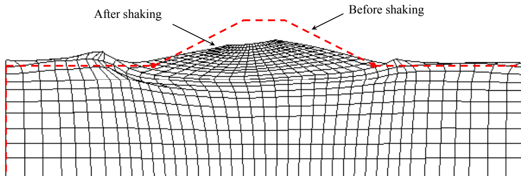
Figure 5.22 Deformed mesh for the case with fully saturated clayey foundation at time t = 25\text{sec} ; magnified 20 times for clarity
