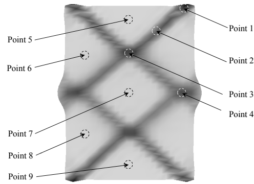
Figure 4.14 Local points inside and outside the shearbands
