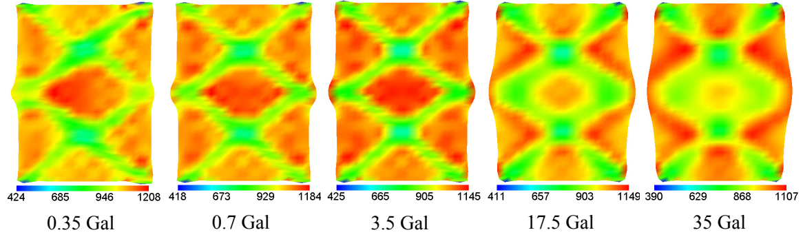
Figure 4.25 Distributions of suction with different accelerations; Unit(kPa); Initial suction P_i^C = 1260 kPa, \varepsilon_a = 20\%
