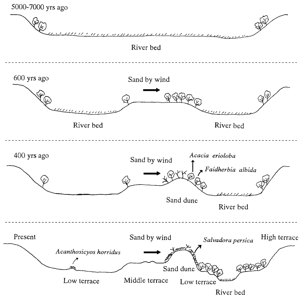
図6 調査地の環境変遷と植生の遷移 Fig. 6. Environmental change and vegetational succession in study area
