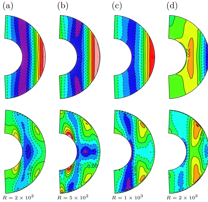
Figure 11. Distributions of mean zonal flows when rigid boundaries are given just below the stable layer. r_i = 0.6667 , r_o = 1.5 , and r_b = 10.5 . The upper and lower panels show the cases of free-slip and no-slip conditions at the top boundary, respectively. Solid lines and red regions indicate the prograde direction, and broken lines and blue regions indicate the retrograde direction (colour online). (a) R = 2 \times 10^2 ; the contour intervals are 5 and 2.5 for the upper and lower panels, respectively. (b) R = 5 \times 10^2 ; the contour intervals are 20 and 5 for the upper and lower panels, respectively. (c) R = 1 \times 10^3 ; the contour intervals are 40 and 10 for the upper and lower panels, respectively. (d) R = 2 \times 10^3 ; the contour intervals are 100 and 20 for the upper and lower panels, respectively.
