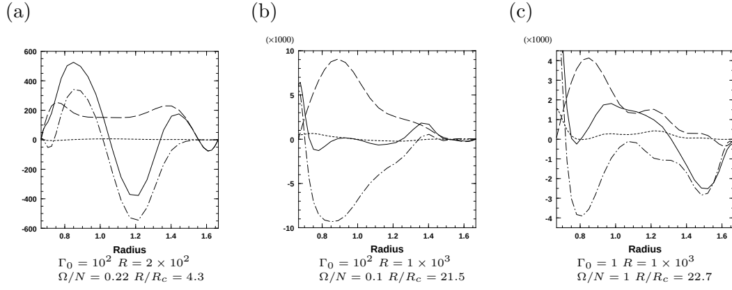
Figure 10. The radial distributions of zonally and temporally averaged angular momentum flux divergences at the equatorial cross section. Solid line denotes \nabla \cdot \mathbf{F}_p + \nabla \cdot \mathbf{F}_r + \nabla \cdot \mathbf{F}_d . Broken, dotted, and broken-dotted lines indicate \nabla \cdot \mathbf{F}_p , \nabla \cdot \mathbf{F}_r , and \nabla \cdot \mathbf{F}_d , respectively. The values of \Gamma_0 and R are the same as those in figure 5 for each case.
