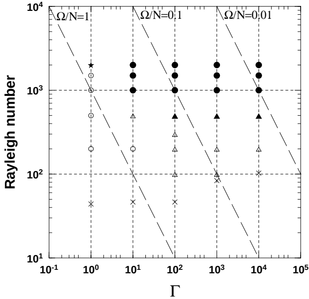
Figure 4. Pattern diagram of the mean zonal flow distributions with respect to the temperature gradient of the stable layer and the Rayleigh number. White and black symbols denote the equatorial prograde and retrograde flows at the outer boundary, respectively. White circles indicate the distributions that are largely uniform along the axis of rotation, as shown in figure 3(a). Crosses denote the critical states. White triangles indicate the distributions that are distorted from the axially uniform fields in the equatorial outer region, as shown in figure 2(b). Black triangles denote the distributions in which the retrograde flows elongate from the equatorial inner to outer regions, as shown in figure 2(b). Black circles indicate the distributions accompanied by the isolated retrograde regions in the equatorial outer stable layer, similar to figure 2(d). The black asterisk indicates the equatorial retrograde flow at the outer boundary produced by angular momentum homogenization.
