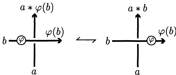
FIGURE 4. Diagrammatic meaning of the condition (K3)
