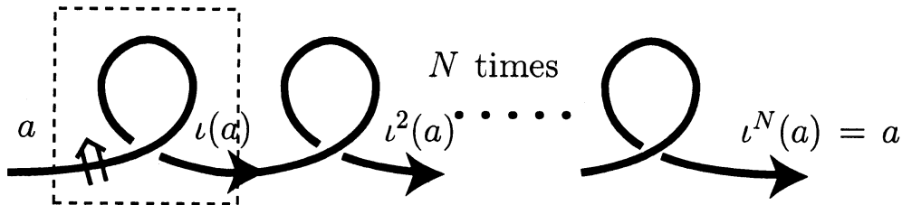
FIGURE 2. Diagrammatic meaning of the rack rank
