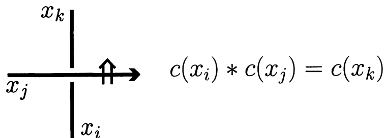
FIGURE 1. Coloring relation at a crossing
