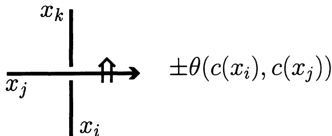
FIGURE 6. Weight at a crossing
