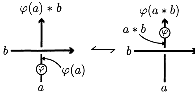
FIGURE 3. Diagrammatic meaning of the condition (K2)
