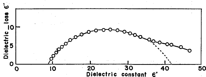
Fig. 8. Complex plane plots of Fig. 7.
