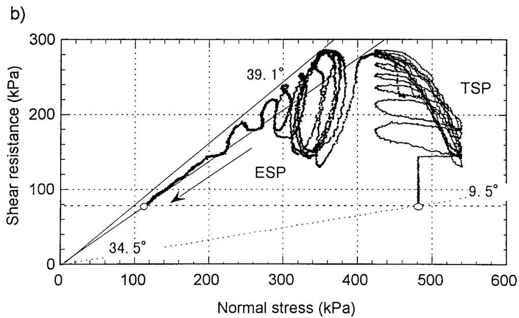
Fig. A-5 Time series data (a) and stress path (b) of 0-F(0.5)-25°
