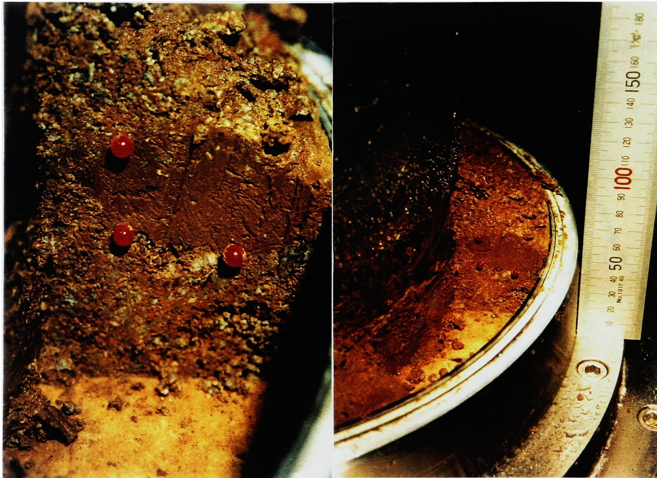
Figure 6.9 Photo of section through the shear zone after the test of Fig. 6.7 (from Sassa et al. 1998).
