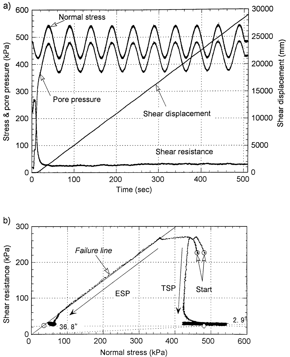
Fig. A-4 Time series data (a) and stress path (b) of 0-F(0.02)-25°
