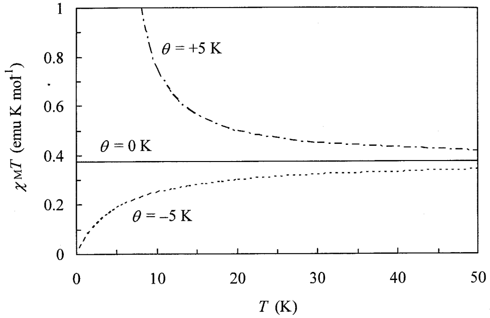
Figure 3. \chi_M T versus T plot for an assembly of 1 mol of species with C = 0.375 \text{ emu K mol}^{-1} obeying the Curie–Weiss law.
