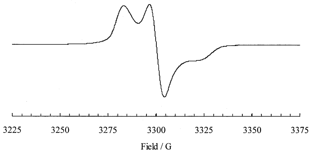
Figure 4. EPR spectrum of 2 after treatment with 2 equiv. of tris(4-bromophenyl)aminium hexachloroantimonate in toluene/ n -butyronitrile = 1:1 at 123 K.
