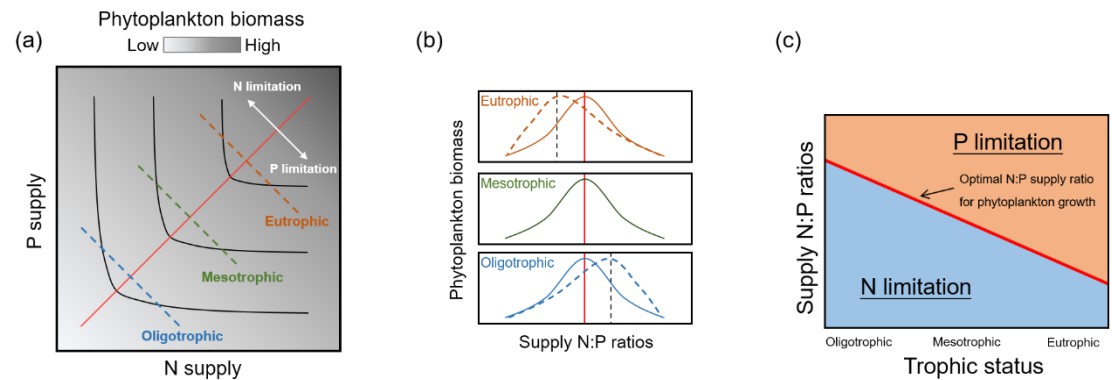
679 680 Figure 1 Hypothesis of the experiment. (a) Hypothetical response of phytoplankton 681 growth under simultaneous co-limitation of nitrogen (N) and phosphorus (P) (Saito et 682 al. 2008; Sperfeld et al. 2012; Sperfeld et al. 2016). Resource-dependent growth 683 isoclines (black lines) indicate equal growth at varying resource availabilities. Colored 684 dash lines represent the trophic statuses. The red line indicates the optimal supply N:P 685 ratio. (b) Unimodal relationship between supply N:P ratios and phytoplankton biomass 686 under different trophic statuses. Solid colored curves represent the hypotheses of 687 previous studies that the position of the peaks are fixed. Dashed colored curves 688 represent the hypothesis of the present study that the peaks will shift with trophic status 689 (i.e., that higher trophic statuses have lower optimal supply N:P ratios, and lower 690 trophic statuses have higher ratios). (c) The predicted development of the optimal N:P 691 ratios, which have a negative relationship with trophic status. Phytoplankton tend to be 692 more P-limited than N-limited at high trophic statuses, and vice versa at low trophic 693 statuses.
