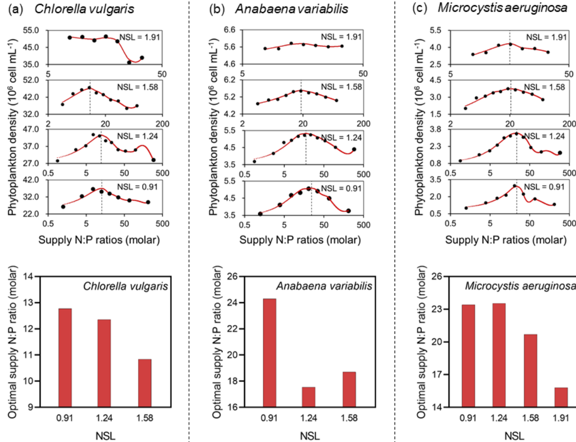
Figure 2 Analytical results of the one-dimensional locally weighted sequential smoothing method (1D-LOESS). Response curves of steady-state phytoplankton biomass (cell density) of (a) C. vulgaris , (b) A. variabilis , and (c) M. aeruginosa to the supply N:P ratios under four NSLs (0.91, 1.24, 1.58, and 1.91). Dashed lines represent the position of the optimal supply N:P ratios calculated using 1D-LOESS fits. The bar graphs summarize the calculated optimal supply N:P ratios under each NSL for the corresponding phytoplankton species.
