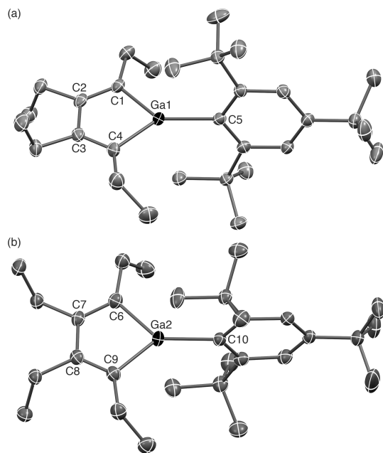
Figure 2. Molecular structure of gallole 1b . (a) Molecule A . (b) Molecule B . Thermal ellipsoids are set at 50% probability level. Hydrogen atoms are omitted for clarity. Selected bond lengths (Å): Molecule A : Ga1–C1 1.976(2), Ga1–C4 1.969(2), Ga1–C5 1.966(2), C1–C2 1.342(3), C2–C3 1.526(3), C3–C4 1.344(3); Molecule B : Ga2–C6 1.974(2), Ga2–C9 1.974(2), Ga2–C10 1.969(2), C6–C7 1.347(3), C7–C8 1.523(3), C8–C9 1.346(3).
