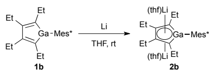
Scheme 2. Synthesis of lithium salt of gallole dianion 2b .
