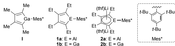
Figure 1. Examples of stable alumoles and galloles. Mes* = 2,4,6-( t -Bu) 3 C 6 H 2 .
