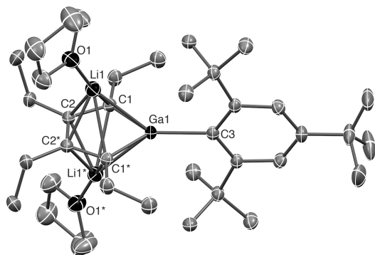
Figure 4. Molecular structure of the lithium salt of gallole dianion 2b . Thermal ellipsoids are set at 50% probability level. Hydrogen atoms are omitted for clarity. Selected bond lengths (Å): Ga1–C1 1.9430(14), Ga1–C3 2.0063(19), C1–C2 1.451(2), C2–C2* 1.434(3), Li1–Ga1 2.554(3), Li1–C1 2.278(3), Li1–C1* 2.297(3), Li1–C2 2.098(3), Li1–C2* 2.113(3), Li1–O1 1.909(3).
