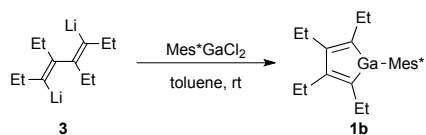
Scheme 1. Synthesis of gallole 1b .
