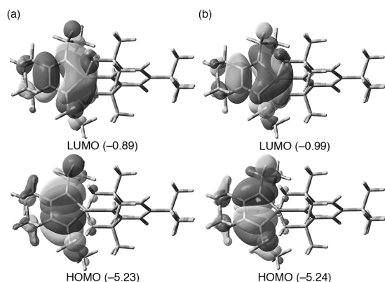
Figure 3. Frontier molecular orbitals of (a) 1a and (b) 1b . Energies are shown in eV.
