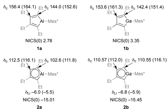
Figure 5. ^{13}C and ^7Li NMR spectral data of the heteroles and the dianions (in C_6D_6 ). Chemical shifts are reported in ppm. Numbers in the parentheses are GIAO-calculated chemical shifts at the B3PW91/6-311+G(2df) level of theory. Nucleus-independent chemical shift (NICS) was calculated at the center of the heterole ring.
