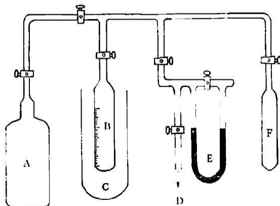
Fig. 1 Apparatus A: storage of acetaldehyde B: glass burette C: jacket D: system of vacuum pump E: manometer F: reaction vessel
