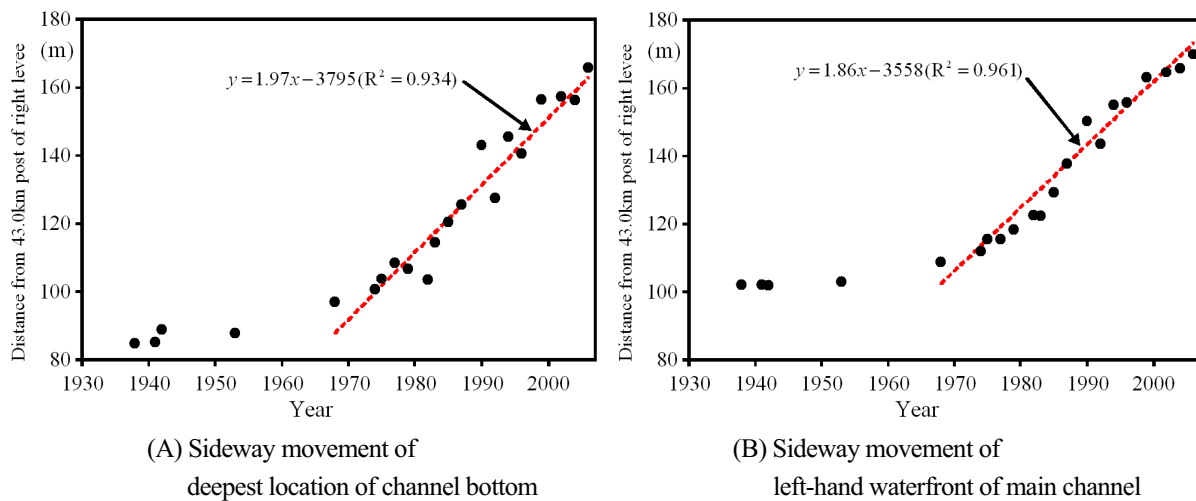
Fig. 12 Time-series data showing evolution of bank erosion
