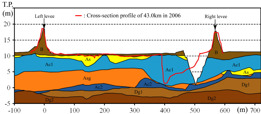
Fig. 13 Cross-section profiles through 43.0km post line is overlain onto a geological profile along Route No.1 bypass (adapted from Kyoto office, MLIT, 1991)
