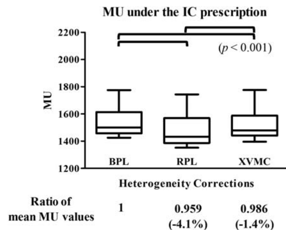
Fig. 4. Box plots of absolute values of monitor units using BPL, RPL, XVMC when 48 Gy was prescribed at the isocenter. The figures in parentheses indicate the percentages of the mean values of monitor units in RPL and XVMC to those in BPL. BPL = the Batho power-law correction, RPL = the radiological path length algorithm, XVMC = the X-ray Voxel Monte Carlo algorithm, MU = monitor units.
