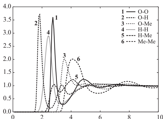
Figure 2.2: Reference RDFs of methanol calculated by MD.
