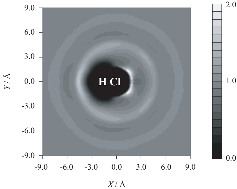
Figure 3.3: 3D solvation structure, G_H(\mathbf{r}) , of the charged HCl model. Solute chloride and hydrogen nuclei are positioned at (0.0, 0.0) and (-1.3, 0.0) , respectively.
