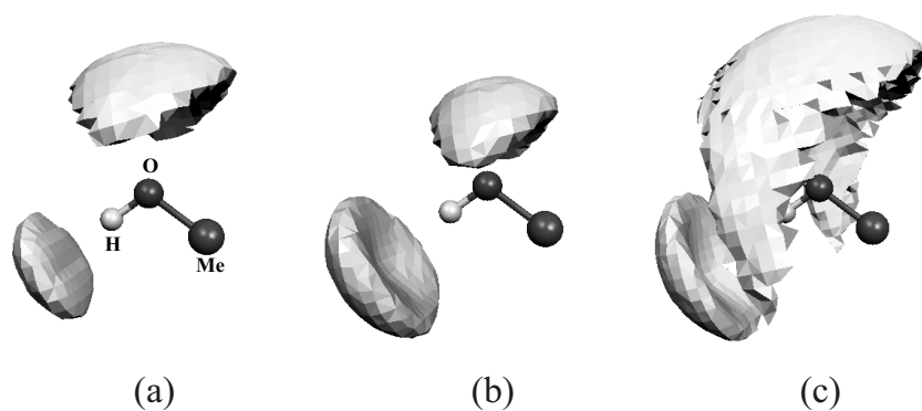
Figure 2.3: Three dimensional SDFs(MD) map of oxygen (a), of hydrogen (b), and of methyl group (c) in methanol. The isosurfaces of SDFs are drawn at n(r) = 3.0 .
