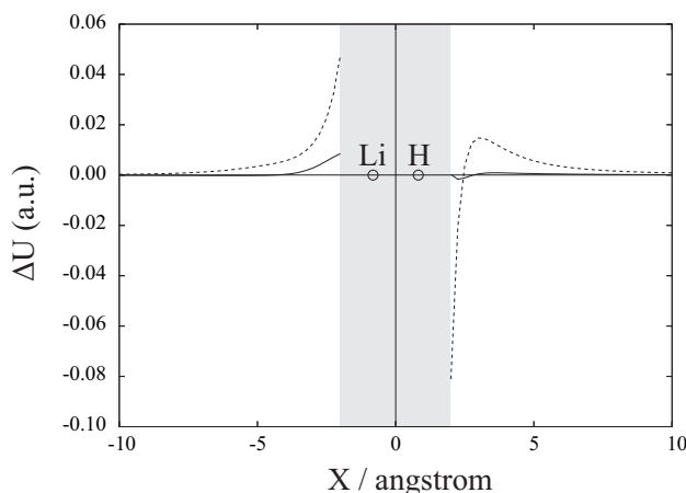
Figure 9.5: The difference of the ESP evaluated by RISM-SCF-SEDD and by the original RISM-SCF from that calculated by QM calculation along HLi bond; solid and dotted line correspond to \Delta U^{SEDD} and \Delta U^{ORG} . Shaded area show the region where the distance from solute site is shorter than the LJ parameter, \sigma/2 .
