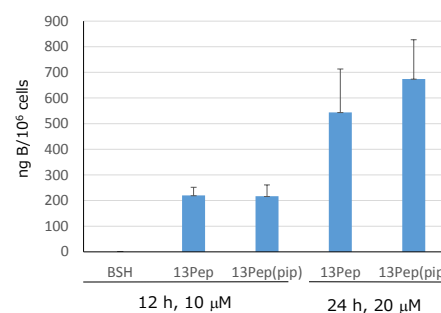
Fig. 2 Intracellular uptake of 13Pep and 13Pep(pip).
