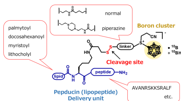
Fig. 1 Structural optimization of pepducin-BSH conjugates.
