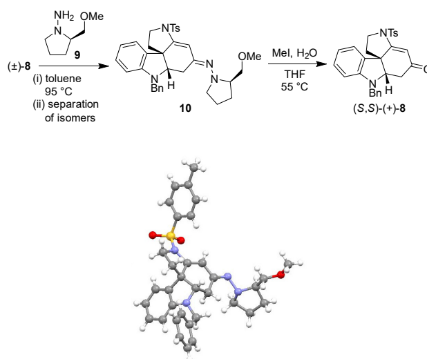
Figure 2. X-ray structure of 10 . There are two crystallographically independent molecules in the single crystal lattices, one of which is shown for clarity.
