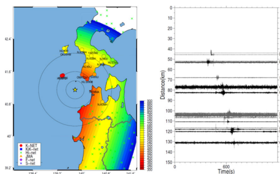
Fig. 13 Map of arrival times and seismic waveform on October 23, 2019. The origin time is 19:30.
