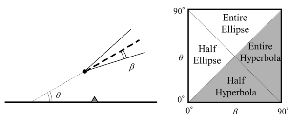
Fig. 5 Sonic boom arrival patterns based on the trajectory of the supersonic object
