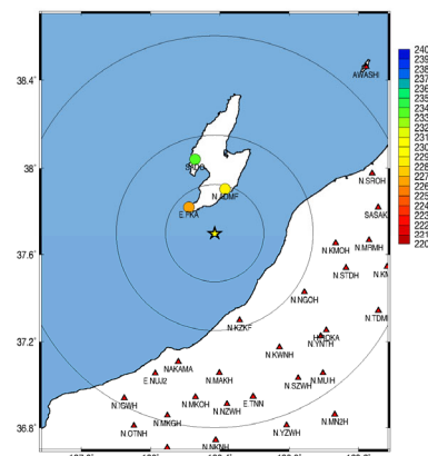
Fig. 12 Map of arrival times on November 7, 2014. The origin time is 16:45.
