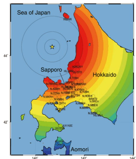
Fig. 17 Map of arrival times of the shock wave on April 26, 2021. The origin time is 20:00.
