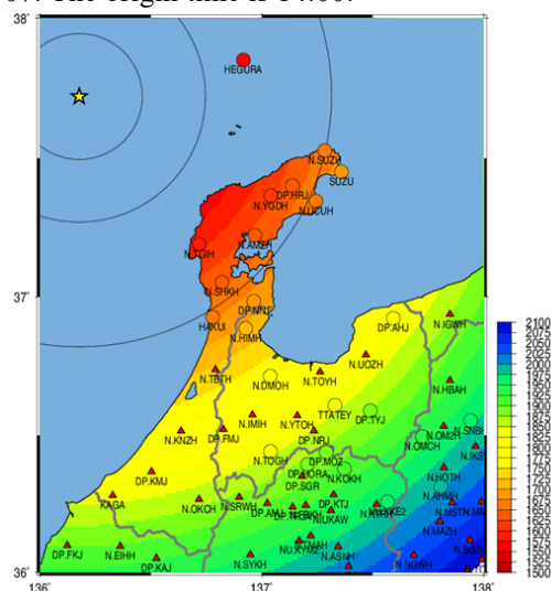
Fig. 9 Map of arrival times of the shock wave on November 27, 2007. The origin time is 14:00.
