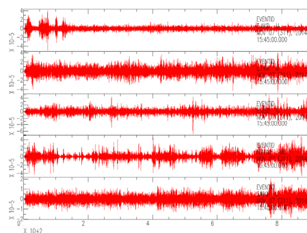
Fig. 10 Seismic waveform (2-8Hz) at 15:45–15:59.
