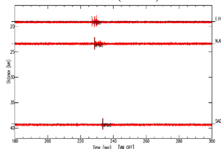
Fig. 11 Seismic waveform ( >1\text{Hz} ) at 16:48–16:50.
