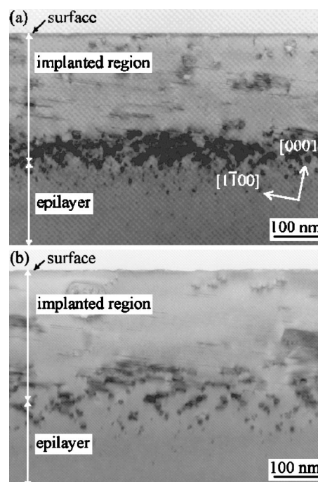
FIG. 4. Cross-sectional TEM images of \text{Al}^+ -implanted (0001) annealed for (a) 1 min and (b) 180 min taken from the [1\bar{2}10] direction. Implant dose for each sample is 3.0 \times 10^{16} \text{ cm}^{-2} .
