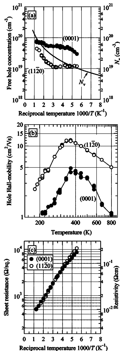
FIG. 5. Temperature dependence of (a) free-hole concentration, (b) hole Hall mobility, and (c) sheet resistance (resistivity) for 4H-SiC (0001) and (1120) implanted with an Al + dose of 3.0 \times 10^{16} \text{ cm}^{-2} and a C + dose of 6.0 \times 10^{15} \text{ cm}^{-2} , obtained from Hall effect measurements. Postimplantation annealing was carried out at 1800 °C for 10 min.
