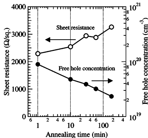
FIG. 3. Annealing-time dependence of sheet resistance and free-hole concentration for \text{Al}^+ -implanted SiC (0001) with a dose of 3.0 \times 10^{16} \text{ cm}^{-2} .
