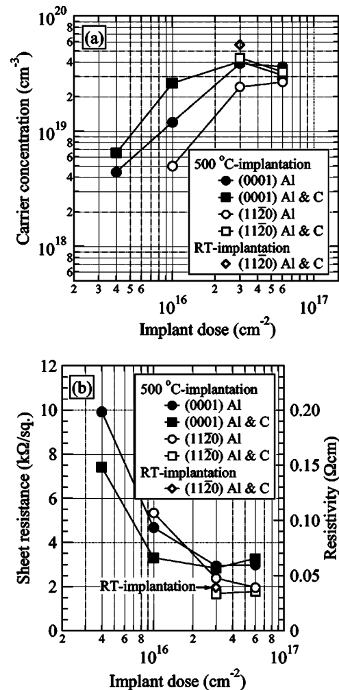
FIG. 1. \text{Al}^+ -dose dependence of (a) free-hole concentration and (b) sheet resistance (resistivity) for 4H-SiC (0001) and (1120) obtained from Hall-effect measurements at RT.
