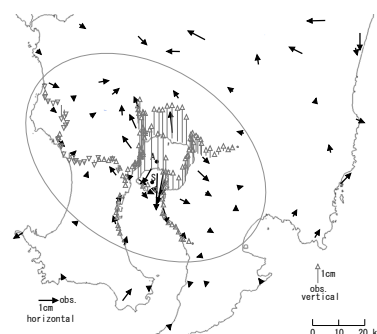
Fig. 2 Ground deformation around Aira caldera during 2017 – 2019 (after Miki et al., 2021).
