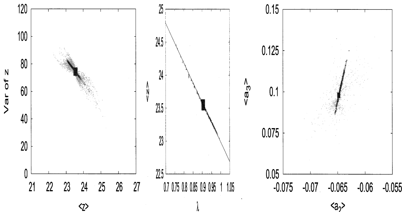
Figure 1: (\langle z \rangle, \text{Var of } z) for each UPO ( N = 1, \dots, 11 ) (green) and each chaotic segment ( N = 11 ) (red) with chaos averages (blue) for the Lorenz system.
