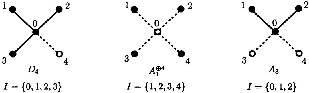
Figure 3: Some strata and their abstract Dynkin types
