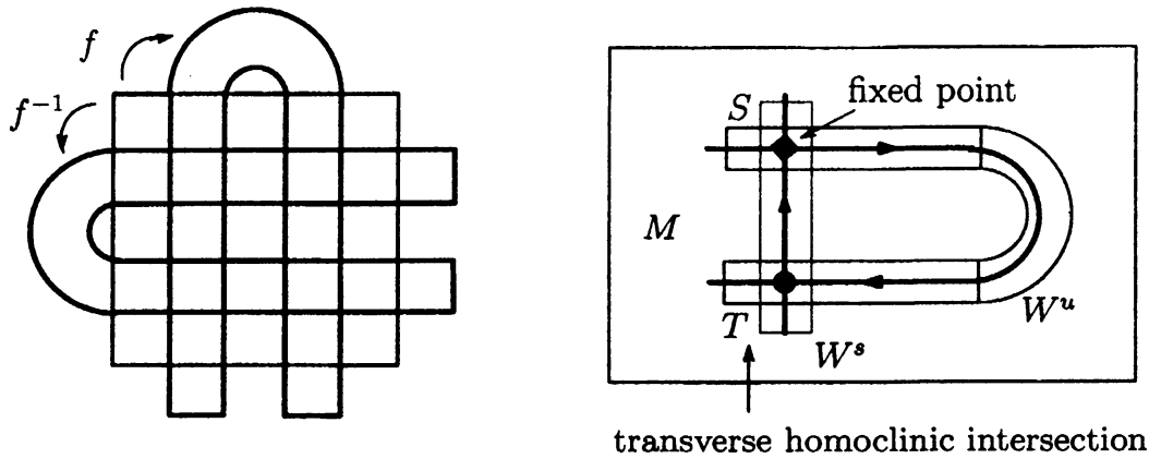
Figure 5: Horseshoe: Smale's geometric model (left) and homoclinic intersection (right).
