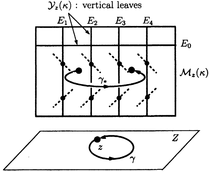
Figure 1: Monodromy map \gamma_* : \mathcal{M}_z(\kappa) \hookrightarrow \mathcal{M}_z(\kappa) along a loop \gamma \in \pi_1(Z, z) .
