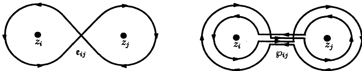
Figure 7: An eight-figured loop (left) and a Pochhammer loop (right).
