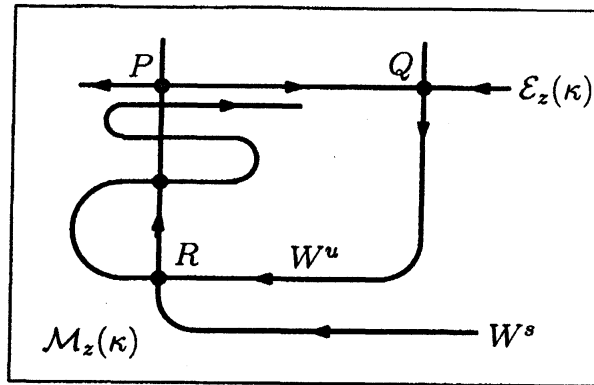
Figure 6: transverse intersection of the stable and unstable curves
