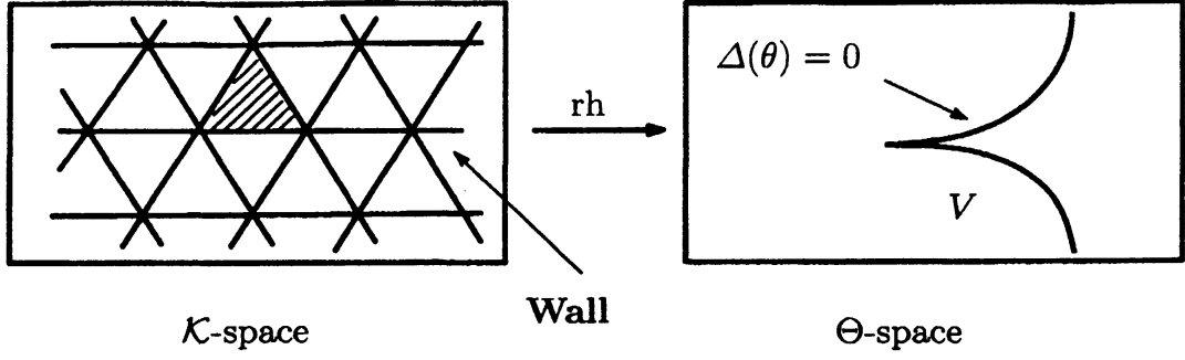
Figure 8: The Riemann-Hilbert correspondence in the parameter level
