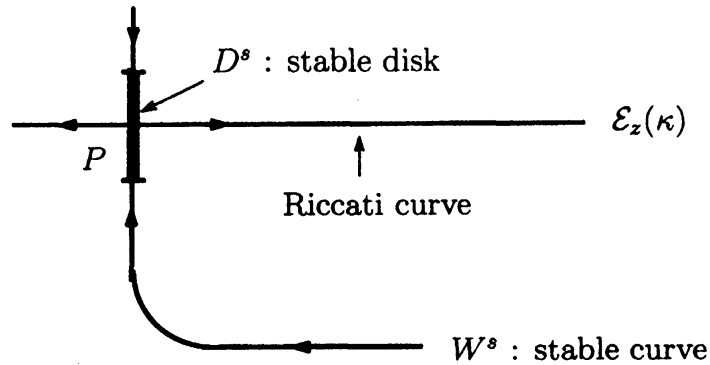
Figure 9: A stable disk D^s
