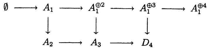
Figure 4: Adjacency relations among the strata
