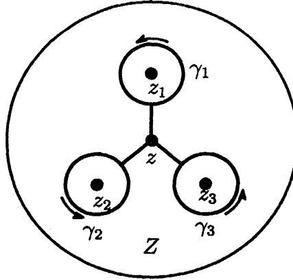
Figure 2: Three basic loops in \pi_1(Z, z) , where z_1 = 0 , z_2 = 1 and z_3 = \infty .
