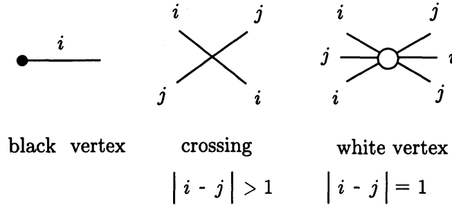
Figure 3: Vertices of a S_d -chart
