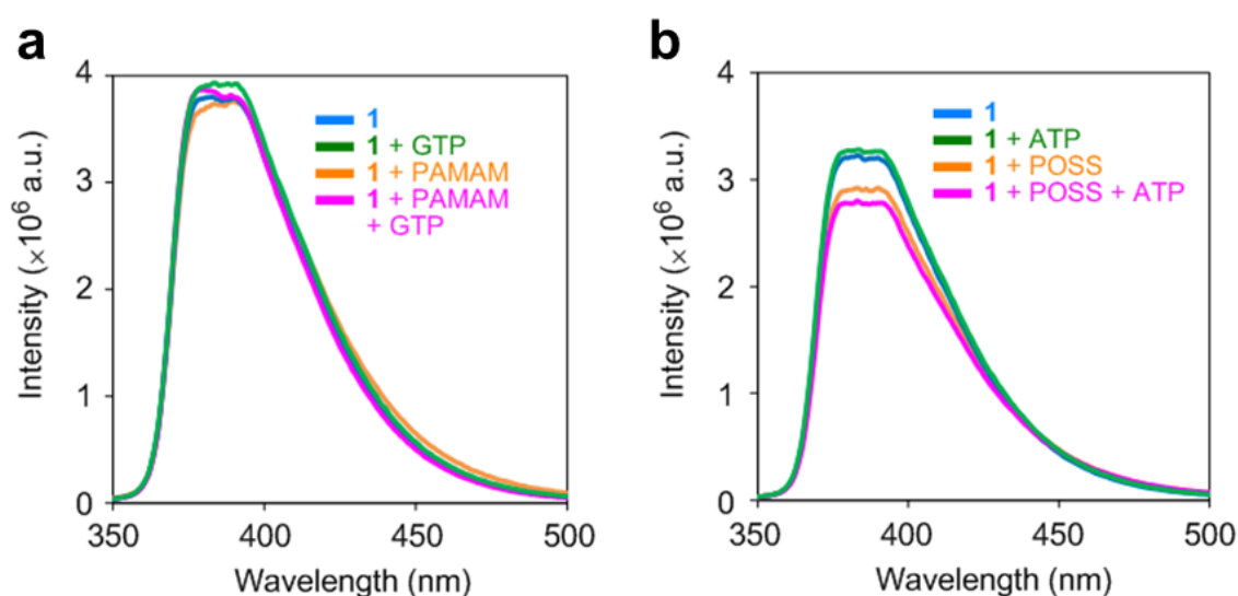
Figure 4. Emission changes of 10 \mu\text{M} 1 in the presence and absence of (a) 100 \mu\text{M} G2 PAMAM dendrimers by adding 100 \mu\text{M} GTP and (b) 100 \mu\text{M} G2 POSS-core dendrimers by adding 100 \mu\text{M} ATP in water at 25 ^{\circ}\text{C} . Excitation wavelength was 330 nm.
