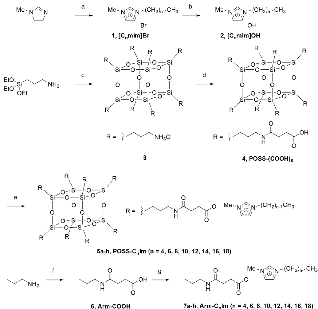
Scheme 1. Synthesis of the ionic compounds a
