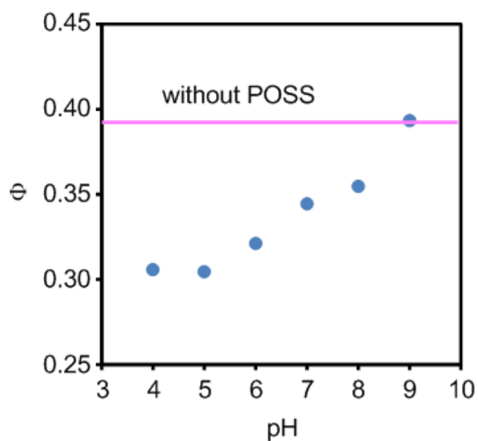
Figure 7. The influence of pH on the quantum yields of the emission from the solutions containing 10 \mu\text{M} 1 , 100 \mu\text{M} G2 POSS-core dendrimer, and 100 \mu\text{M} GTP in 50 mM sodium phosphate buffer at 25 °C. Excitation wavelength was 330 nm.
