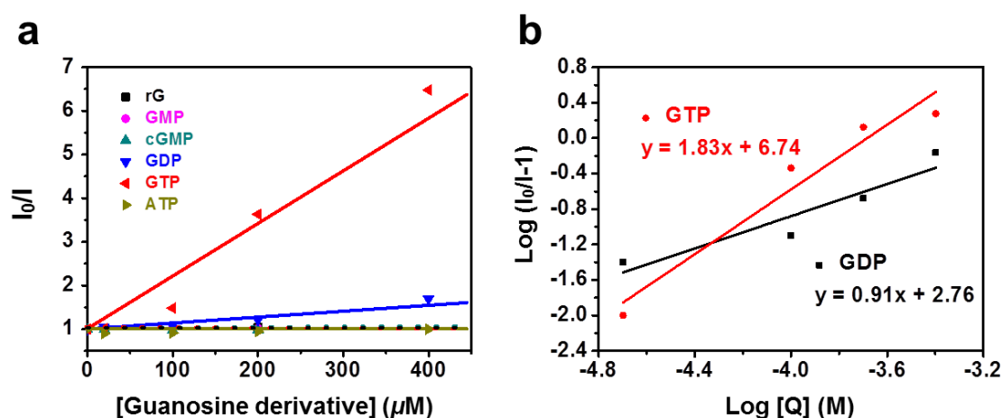
Figure 5. (a) Stern–Volmer plots with the solution containing 20 \mu\text{M} naphthyridine ligands in the POSS-N network polymers by adding various kinds of guanosine nucleotides. (B) The plots for determining the binding constants between the naphthyridine ligands in the POSS-N network polymers and guanosine nucleotides according to the above equation. The slopes represent the number of the binding guanosine nucleotides. The y-intercepts represent the \log K_A values. The lines were prepared with the least-square method. R^2 is determination coefficient.
