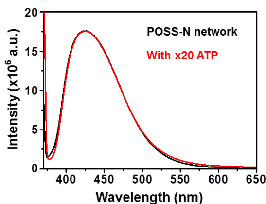
Figure 4. Emission change of 20 \mu\text{M} naphthyridine ligands in the POSS-N network polymer by adding 400 \mu\text{M} of adenosine triphosphate (ATP) in PBS buffer solution (pH 7.4) at 25 ^{\circ}\text{C} . Excitation wavelength was 364 nm.
