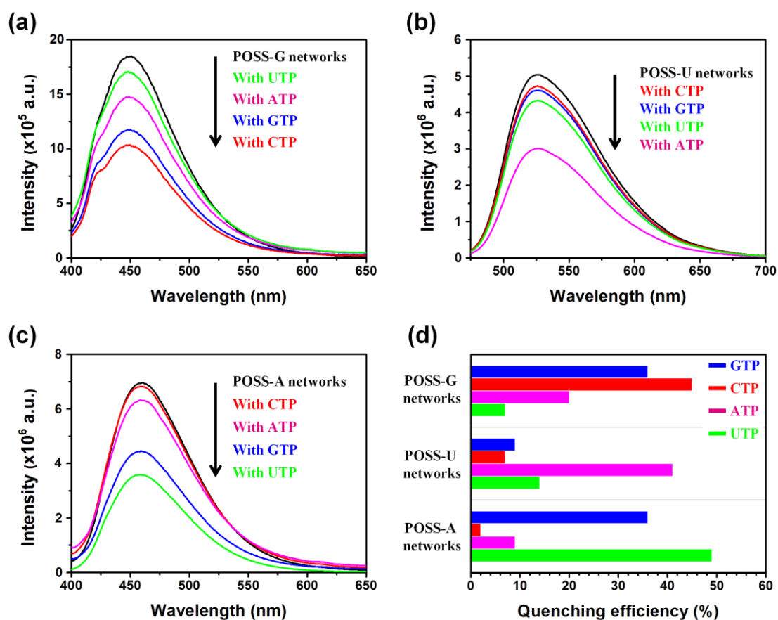
Figure 6. Fluorescence spectra of (a) POSS-G networks, (b) POSS-U networks, and (c) POSS-A networks in the absence and presence of different flanking nucleotides. (d) Comparison of fluorescence quenching efficiencies of POSS network ligands in the absence and presence of nucleobases. [Ligand] = 20 \mu M, [Nucleobase] = 200 \mu M in PBS buffer solution (pH 7.4) at 25 ^{\circ} C.
