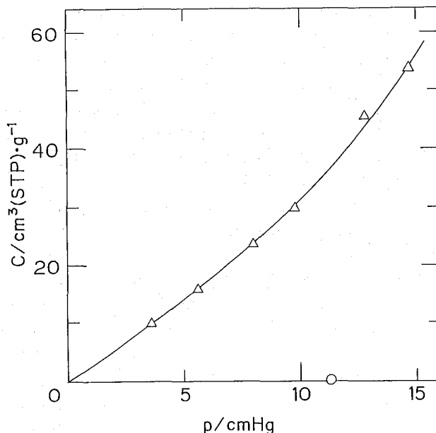
Fig. 1. Sorption isotherms of gas and vapor in poly(vinyl acetate) at 30°C. ○: \text{CO}_2 , △: acetone vapor.
