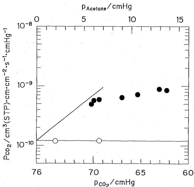
Fig. 3. Dependence of permeability coefficient for carbon dioxide on partial pressure at 30°C. ○: \text{CO}_2 , pure; ●: \text{CO}_2 , mixture; —(thick): \text{CO}_2 , mixture, calculated from Eq. (4).
