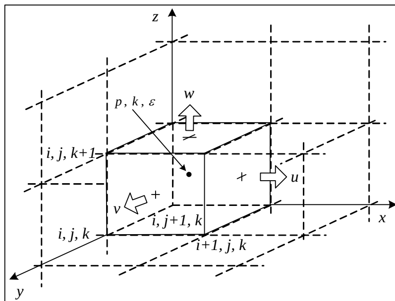
Figure 3.2. Arrangement of hydraulic variables on full staggered grid
