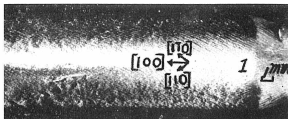
Fig. 8. Optical micrograph of the side surface (001) of the specimen (99.98 % pure tin) grown at 2.8 mm/min and 15°/cm.
