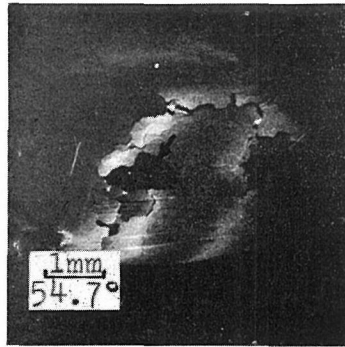
Fig. 15. X-ray micrograph of the cross section (001) of the specimen (99.98 % pure tin) grown in parallel to [001] at 2.5 min and 45°/cm. Fe K \alpha , reflecting plane : (103).
