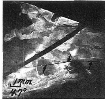
Fig. 14. X-ray micrograph of the side surface (100) of the specimen (99.98% pure tin) in parallel to [001] at 0.13 mm/min and 45^{\circ}/\text{cm} . Fe K\alpha , reflecting plane : (301).
