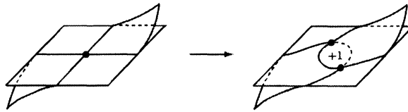
FIGURE 4. Local replacement of W_f .
