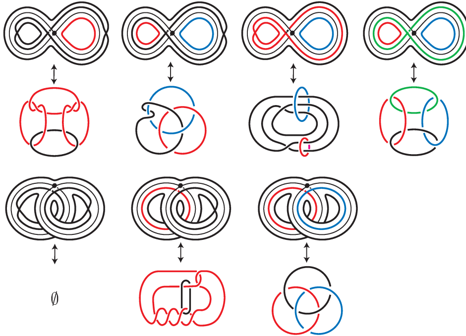
FIGURE 8. The correspondence between links in S^3 and the neighborhoods of the singular sets of branched polyhedra having a single vertex.
