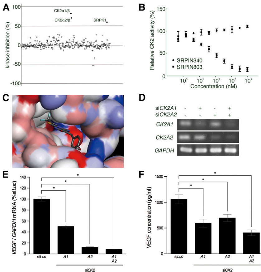
Fig. 4. SRPIN803 is a dual inhibitor of SRPK1 and CK2. (A) Scatter plots of the 306-kinase panel of SRPIN803 (2.5 \mu M). Black dots indicate greater than 50% inhibition. (B) SRPIN803 inhibited CK2 activity with an IC_{50} value of 203 nM, whereas SRPIN340 did not inhibit the enzyme. (C) A docking model of SRPIN803 bound to the ATP-binding pocket of CK2 \alpha (Supplemental PDB file 2). (D) Semiquantitative PCR analysis to determine expression of CK2A1 and CK2A2 in the ARPE-19 cells. siRNAs against CK2A1 and CK2A2 reduced the corresponding mRNA levels, relative to treatment with control siRNA against luciferase. GAPDH was used as an internal control. (E and F) Treatment with siRNA against either CK2A1 or CK2A2 significantly suppressed expression of VEGF mRNA and decreased the level of secreted VEGF protein, relative to the treatment with the control. * P < 0.01 . (E) Quantitative PCR analysis of total VEGF mRNA of the ARPE-19 cells transfected with siRNAs (means \pm S.E.M. of the results from four experiments performed in duplicate). (F) Enzyme-linked immunosorbent assay of secreted VEGF protein in the culture supernatants of the ARPE-19 cells transfected with siRNAs (means \pm S.E.M. of three independent experiments).
