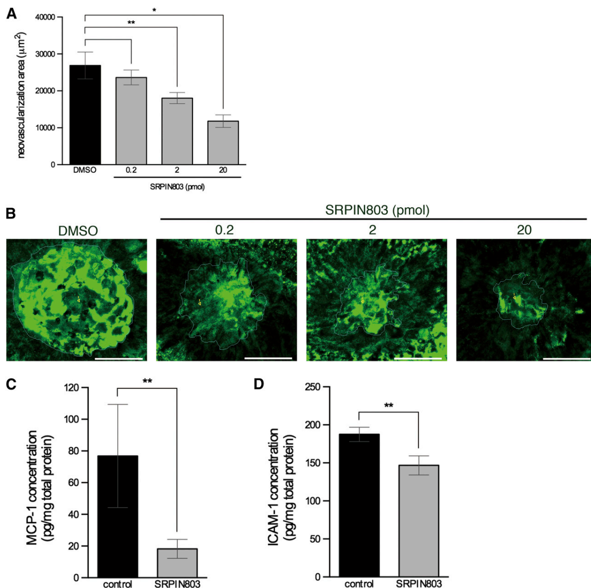
Fig. 5. SRPIN803 suppresses choroidal neovascularization in laser-induced model mice. (A and B) Intravitreal injection of SRPIN803 suppressed choroidal neovascularization. (A) Choroidal flat mounts were prepared from model mice 7 days after laser photocoagulation combined with intravitreal injection of 0.1% DMSO or SRPIN803 (0.20, 2.0, 20 pmol). The areas of choroidal neovascularization lesions in the flat mounts were quantitated [means \pm S.E.M., n (number of neovascular lesions) = 17–26; * P < 0.01; ** P < 0.05; ^{\dagger}P = 0.43]. (B) Representative micrographs of neovascular lesions prepared in (A). Scale bar, 100 \mu\text{m} . (C and D) Reduction of inflammatory molecules by injection of SRPIN803. Bars indicate average protein levels of MCP1 (C) and ICAM1 (D) in retinal pigment epithelium and choroid obtained from model mice 3 days after laser photocoagulation combined with intravitreal injection of 0.1% DMSO or SRPIN803 (20 pmol). Protein levels were measured with enzyme-linked immunosorbent assay and normalized to total protein levels [means \pm S.E.M., n (number of eyes) = 6; ** P < 0.05].
