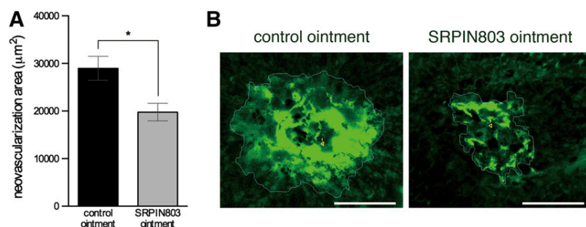
Fig. 6. SRPIN803 ointment suppresses choroidal neovascularization. (A and B) Treatment with ointment containing SRPIN803 (final concentration, 10%) suppressed choroidal neovascularization. (A) Quantitative analysis of the area of neovascularization [means \pm S.E.M., n (number of neovascular lesions) = 18 for the control, n = 26 for SRPIN803; *P < 0.01 ]. (B) Representative micrographs of neovascular lesions prepared in (A). Scale bar, 100 \mu\text{m} .
