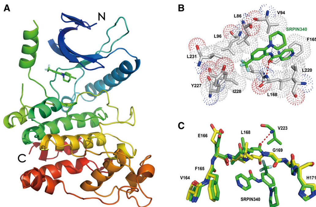
Fig. 1. Crystal structure of the SRPK1/SRPIN340 complex. (A) Overall structure. SRPK1 and SRPIN340 are shown in ribbon mode and stick mode, respectively. SRPIN340 binds to the ATP-binding pocket of SRPK1 (PDB ID 4WUA). C, carboxy terminus; N, amino terminus. (B) Stick representation of the inhibitor-binding site of the SRPK1/SRPIN340 complex. The red dotted line indicates a hydrogen bond. A space-filling model is illustrated by the dots surrounding the stick representation. (C) The peptide flip around Leu168–Gly169. Residues Val164–His171 and Val223 are shown in stick representation. The structures illustrated are SRPK1 without ligand (PDB ID 1WAK), shown in yellow, and SRPK1 with SRPIN340, shown in green. The red dotted line indicates a hydrogen bond.
