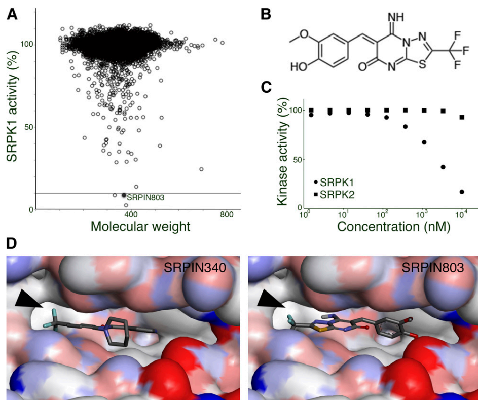
Fig. 2. Identification of SRPIN803 as an inhibitor of SRPK1. (A) Relative in vitro activities of SRPK1 in the presence of small molecules (10 \mu M). A total of 9511 compounds were screened. The top three compounds that inhibited SRPK1 activity to below 10% of the DMSO control are shown in the scatter plot. (B) Chemical structure referred to as SRPIN803. (C) SRPIN803 inhibits the kinase activity of SRPK1 with an IC_{50} value of 2.4 \mu M but does not inhibit SRPK2. (D) A docking model for SRPIN803 to SRPK1 (right, Supplemental PDB File 1), compared with the same view of the crystal structure of the SRPK1/SRPIN340 complex (left, PDB ID 4WUA). The arrowhead indicates the trifluoromethyl group.
