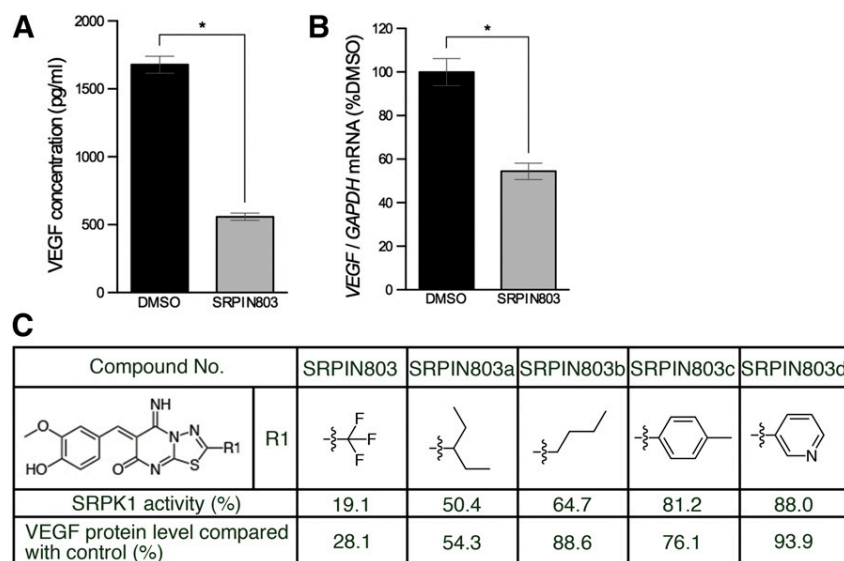
Fig. 3. SRPIN803 suppresses VEGF production. (A and B) Treatment with SRPIN803 decreases total VEGF protein and VEGF mRNA relative to the treatment with 0.1% DMSO. * P < 0.01. (A) Enzyme-linked immunosorbent assay (ELISA) of total VEGF protein in culture supernatants of ARPE-19 cells treated with SRPIN803 (10 \mu M) (mean \pm S.E.M. of four independent experiments). (B) Quantitative PCR analysis of total VEGF mRNA of the ARPE-19 cells treated with SRPIN803 (10 \mu M) (mean \pm S.E.M. of the results of four experiments performed in triplicate). (C) Structural requirements for SRPK1 inhibition by SRPIN803. The chemical structures of SRPIN803 and its derivatives are shown. IC_{50} values of these derivatives were calculated by in vitro kinase assay. The levels of secreted VEGF protein in culture supernatants of ARPE-19 cells treated with the derivatives (final concentration, 10 \mu M) were measured by ELISA.
