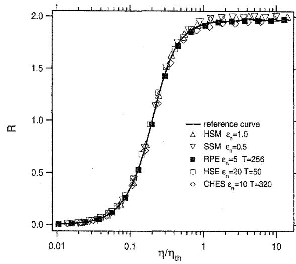
图 4: Time-reversal characteristics of all the models examined. Case of the perpendicular shift perturbation. All curves are those obtained as the converged curves in a large limit of T . CHES denotes a result for CHE with stochastic perturbation. The bold line is the reference curve.
