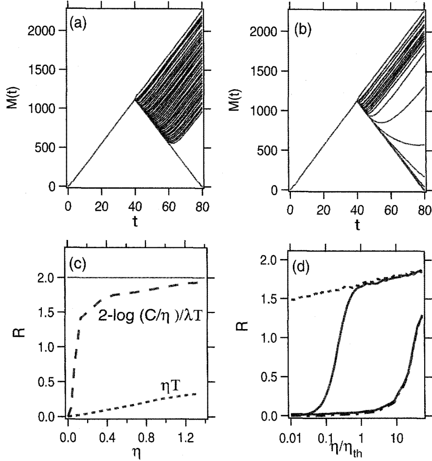
图 1: Typical time-reversal tests for the normal diffusion in (a)classical and (b)quantum SM with K = 6 , \hbar = \frac{2\pi 121}{217} , where \eta is decreasing geometrically, and the delay time increases linearly in (a). (c) Schematic illustration of time-reversal characteristics \mathcal{R}_{cl} as a function of the perturbation strength for some typical cases in classical dynamics. See the main text for the explanation of the function form. (d) Typical time-reversal characteristics for quantum (red full) and classical(blue broken) SM with normal diffusion obtained by time-reversal tests. The bottom curve denotes the typical result for the quasi-integrable quantum and classical SM. Note that the horizontal axis is in logarithmic scale in arbitrary unit.
