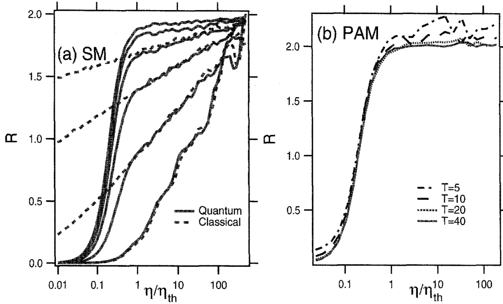
FIG 2: Time-reversal characteristics of (a) quantum (solid) and classical (broken) SM and (b) PAM, as functions of the scaled perturbation strength \eta/\eta_{th} at T = 5, 10, 20, 40 (in order from below in (a) and as marked in (b)). K = 6 , \hbar = \frac{2\pi 121}{2^{17}} for SM and W = 1.0, M = 3, \epsilon = 0.5 for PAM. In (a) the classical time-reversal characteristics agrees with Eq.(19).
