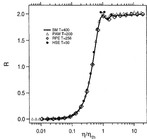
图 5: Time-reversal characteristics of several models examined. Case of parallel shift perturbation. All curves are those obtained as the converged curves in a large limit of T . The bold line is the reference curve.
