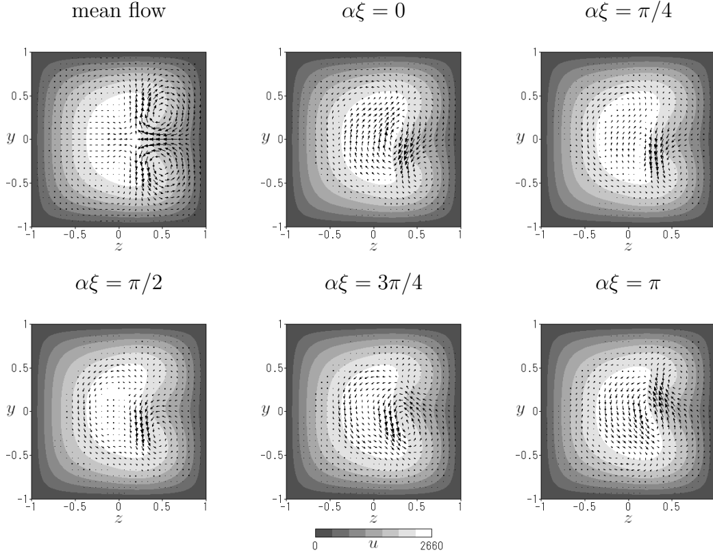
Figure 3.6: Mean flow \bar{U} (top-left) and images of the total flows \mathbf{u} along \xi of the S -symmetric solution with \alpha = 0.7 at Re = 3000 ( Re_b = 1342 ). The velocity components are shown on the y - z plane (arrows) and along the x -direction (grey scale). \xi = x - ct .
