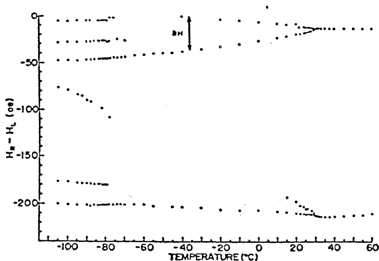
Fig. 2. The temperature dependence of the second order quadrupolar shifts of ^{87}\text{Rb} central lines measured from 60 to -105^\circ\text{C} . The sample was oriented with its b axis parallel to the magnetic field.
