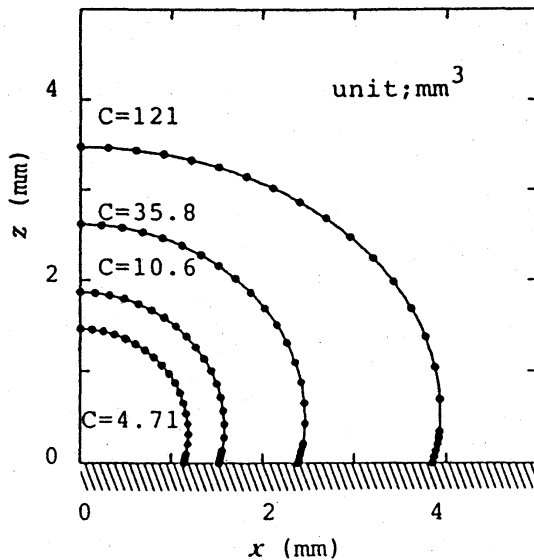
Fig.6 Upward droplets
