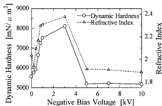
FIG. 6. Dynamic hardness and refractive index of the DLC film as a function of negative bias voltage.
