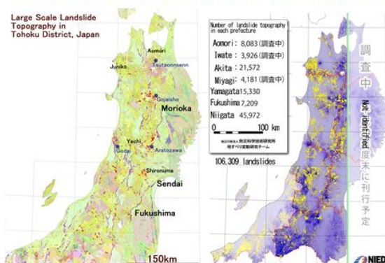
Geology and landslide area in Tohoku, Northeastern Japan
