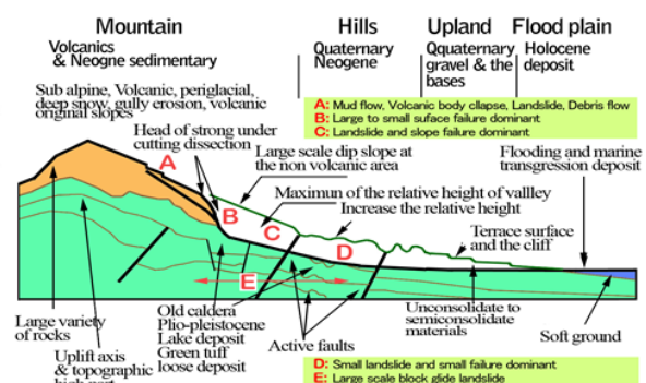
Geo-environmental setting and the landslide types in the Tohoku region as a typical Island ark
