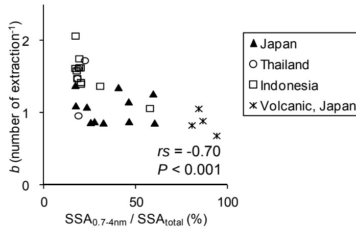
FIG. 4. Relationship between the percentage of SSAs of micro- and meso-pores (0.7–4 nm) ( SSA_{0.7-4 \text{ nm}} ) relative to the total SSA ( SSA_{\text{total}} ) and the constant b representing phosphate release rate using an anion exchange membrane.
