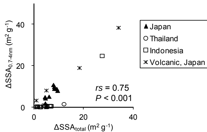
FIG. 6. Relationship between the decrease in total specific surface area ( \Delta SSA_{\text{total}} ) and the decrease in SSAs of micro- and meso-pores (0.7–4 nm) after phosphate sorption treatment ( \Delta SSA_{0.7-4 \text{ nm}} ).
