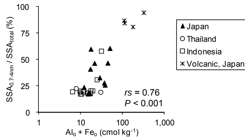
FIG. 3. Relationship between acid oxalate-extractable Al and Fe contents ( Al_0 and Fe_0 ) and the percentage of SSAs of micro- and meso-pores (0.7–4 nm) ( SSA_{0.7-4\ nm} ) relative to the total SSA ( SSA_{total} ).
