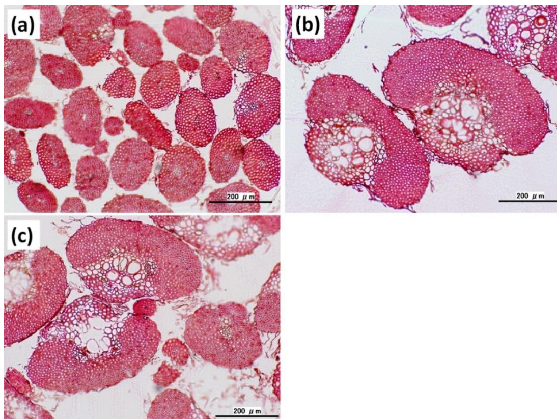
Figure 6.5 Transverse sections of fibrovascular bundles taken from inner (a) , middle (b) , and outer layers (c) of one sheet of leaf sheath, showing vessels and phloem tissue accompanied by fibers in each fibrovascular bundle. (Zhai et al. 2012)
