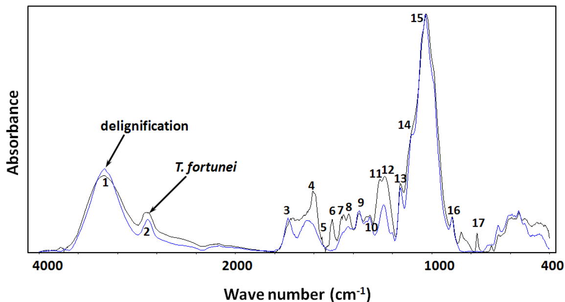
Figure 3.7 FTIR spectra of T. fortunei fibrovascular bundles and delignified fibrovascular bundles.
