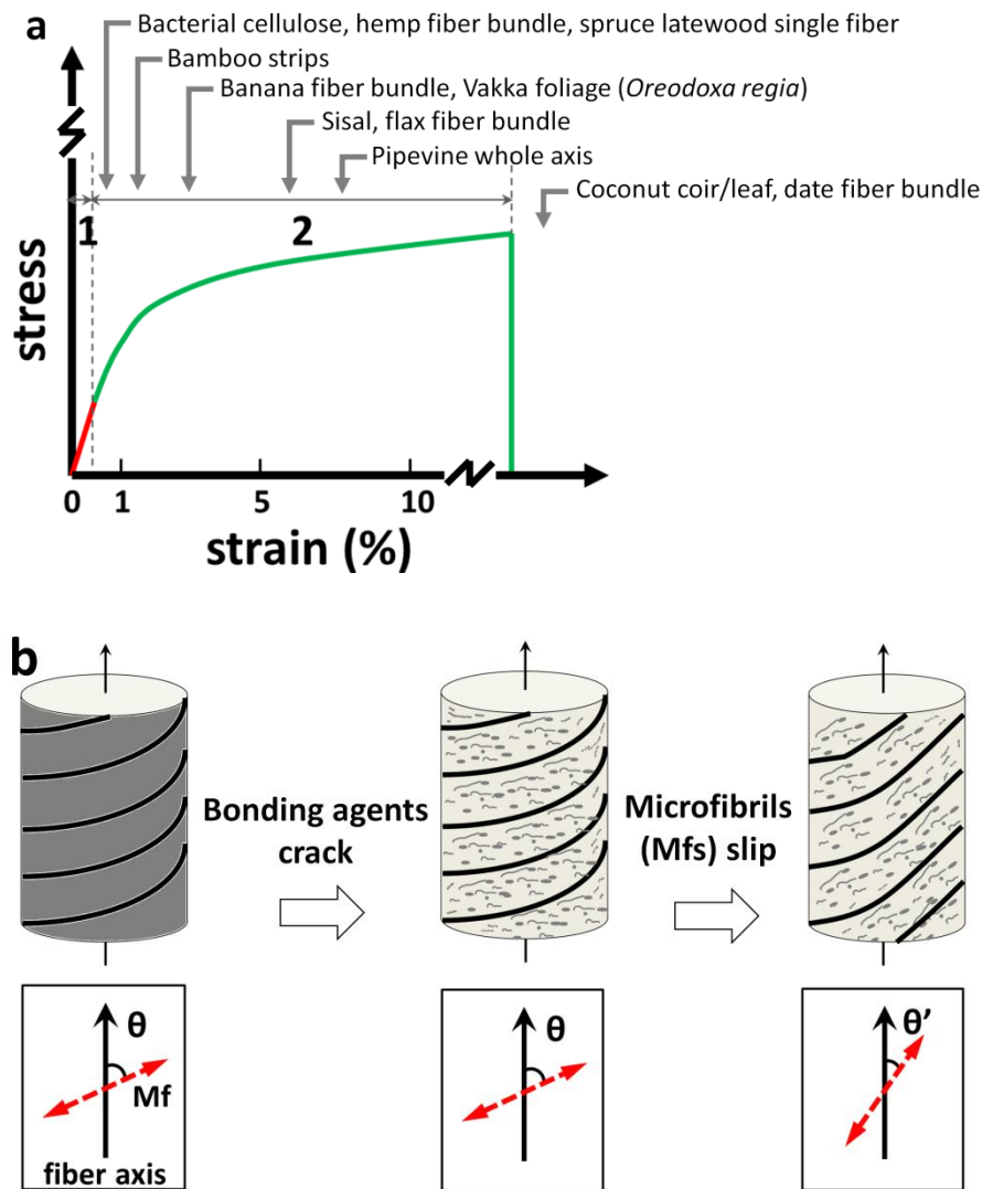
Figure 7.6 Illustration of elastic and plastic deformation behavior. (a) S-S curve shows elastic deformation region (1) and plastic deformation region (2) of different biomass materials. (b) Cell wall structural change during elastic and plastic deformation behavior.
