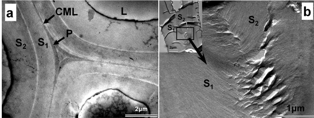
Figure 4.3 Electron micrographs of the windmill palm leaf fibers. (a) Transverse section of a two-layered secondary wall of windmill palm leaf fibers. (b) Enlargement of the fiber cell tip on the oblique section, demonstrating microfibril orientation in the two layers of the secondary wall. CML: compound middle lamella; L: lumen; P: primary wall; S_1 , S_2 : outmost and inner layers of the secondary wall (Zhai et al. 2013).
