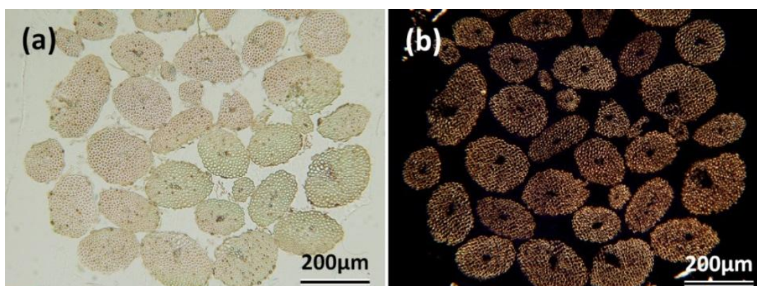
Figure 6.6 Transverse sectional image of fibrovascular bundles in the inner layer observed by transmitted- (a) and polarized-light (b) . The noticeable dark region near the center of each fibrovascular bundle in (b) is the area occupied by vessels and phloem tissue. (Zhai et al. 2012)
