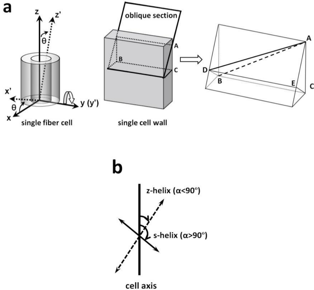
Figure 2.8 Illustration of the relationship between real MFA and the apparent MFA. --a: An orthogonal co-ordinate system ( x, y, z ) is set. The ( x, y, z ) axis was rotated by \theta degree ( \angle CAE ) around the y -axis to give the ( x', y', z' )-axes. The oblique section was located in the y'-z' plane. The oblique section is partially enlarged for displaying the microfibril localization. AB is the cellulose microfibril localization at the longitudinal section of a cell wall. The real MFA is \angle BAC = \alpha to the cell axis. On the oblique section, the angle between AD and the cell axis is visible using polarized light microscopy, which is the apparent MFA ( \angle DAE = \alpha' ) that we sought to measure. --b: Definition of Microfibrils orientation (z-helix or s-helix) related with MFA ( \alpha ). The double arrow lines indicate microfibrils.
