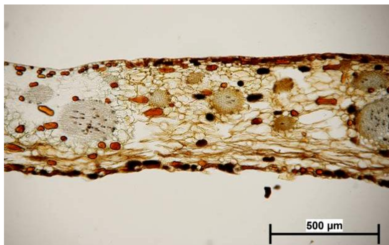
Figure 3.11 Transverse section of No. 18 leaf sheath of T. fortunei showing the distribution of vascular bundles in different size. Bar=500μm.
